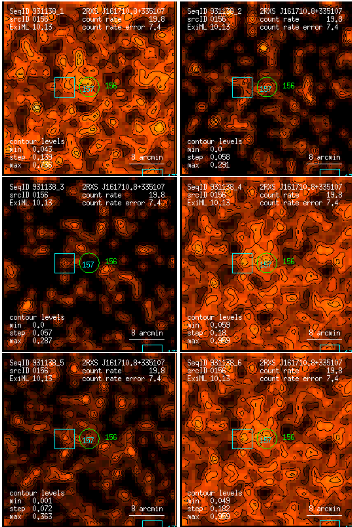
Figure 156: RASS 931138: detection 0156: band rate images, Gaussian filter: (1) PSPC channels 11 – 41, (2) 52 – 90, (3) 91 – 201, (4) 11 – 235, (5) 52 – 201, (6) 11 – 201. Broad band rates in counts/ks. Band rate contour levels in counts/ks/arcmin 2 .
