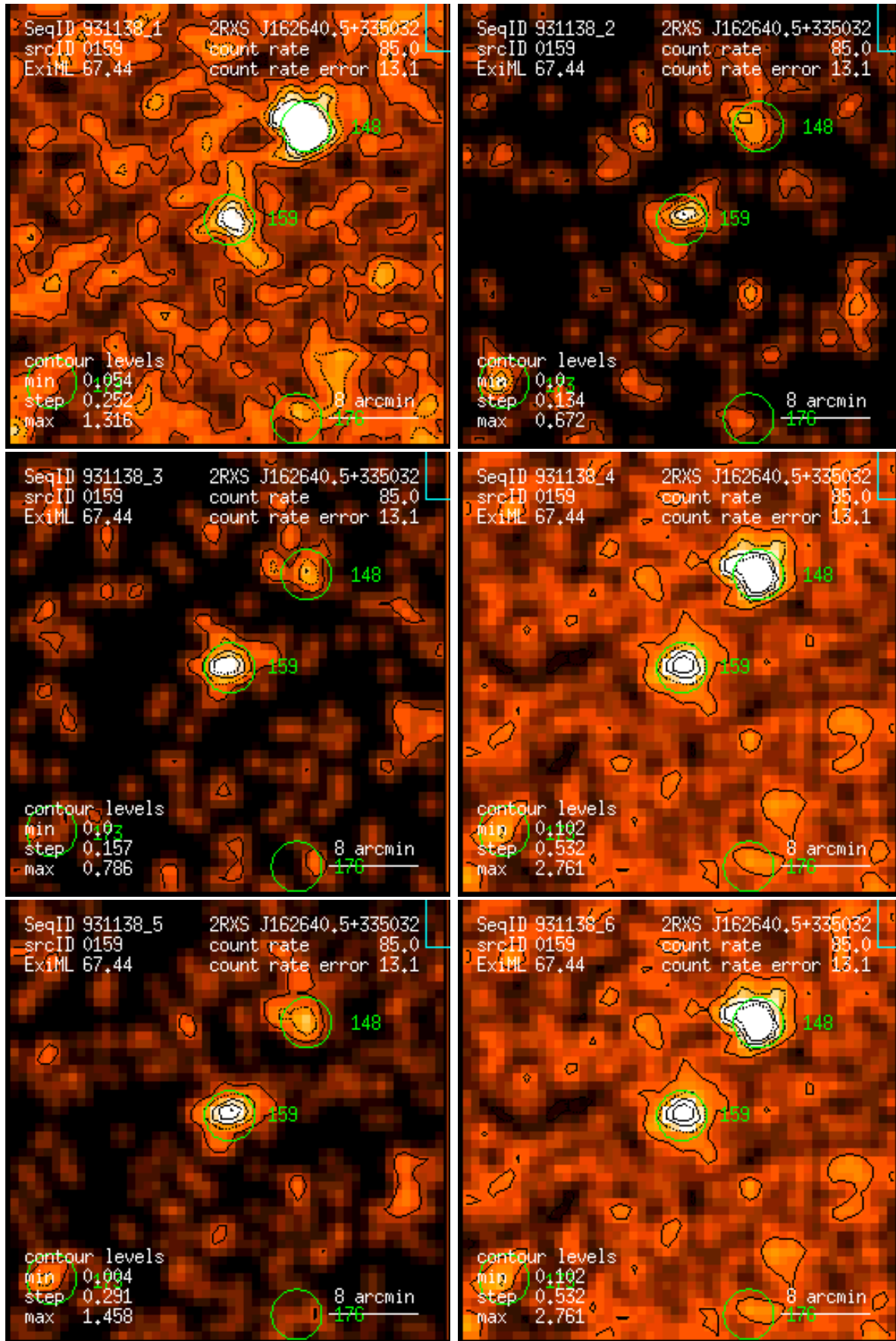
Figure 159: RASS 931138: detection 0159: band rate images, Gaussian filter: (1) PSPC channels 11 – 41, (2) 52 – 90, (3) 91 – 201, (4) 11 – 235, (5) 52 – 201, (6) 11 – 201. Broad band rates in counts/ks. Band rate contour levels in counts/ks/arcmin 2 .
