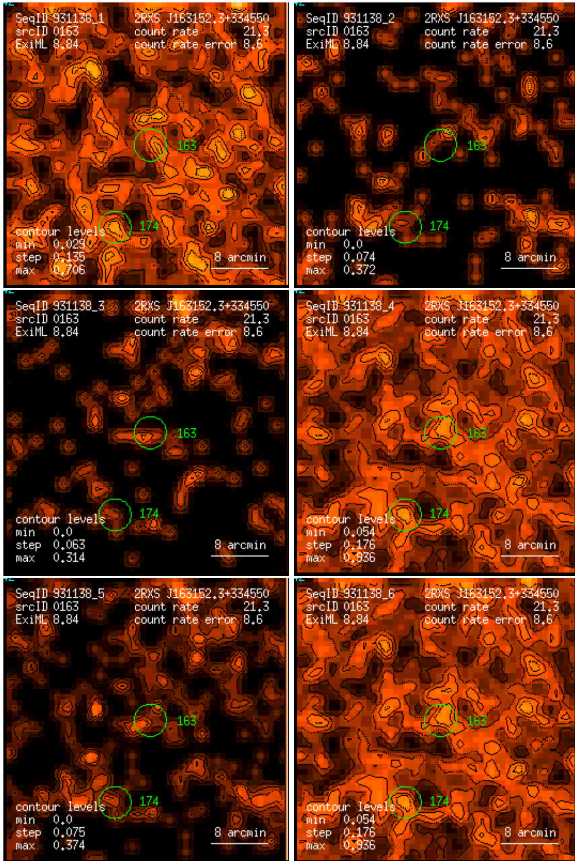
Figure 163: RASS 931138: detection 0163: band rate images, Gaussian filter: (1) PSPC channels 11 – 41, (2) 52 – 90, (3) 91 – 201, (4) 11 – 235, (5) 52 – 201, (6) 11 – 201. Broad band rates in counts/ks. Band rate contour levels in counts/ks/arcmin 2 .
