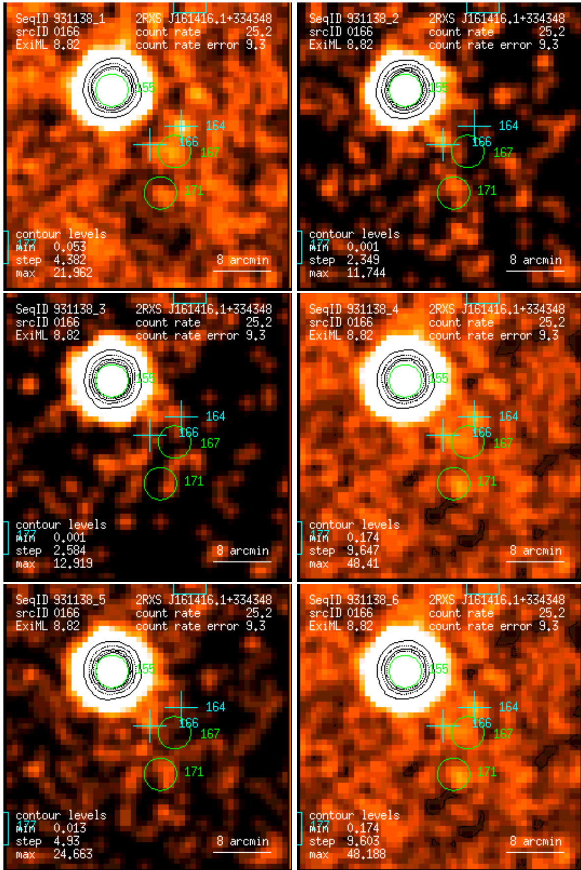
Figure 166: RASS 931138: detection 0166: band rate images, Gaussian filter: (1) PSPC channels 11 – 41, (2) 52 – 90, (3) 91 – 201, (4) 11 – 235, (5) 52 – 201, (6) 11 – 201. Broad band rates in counts/ks. Band rate contour levels in counts/ks/arcmin 2 .
