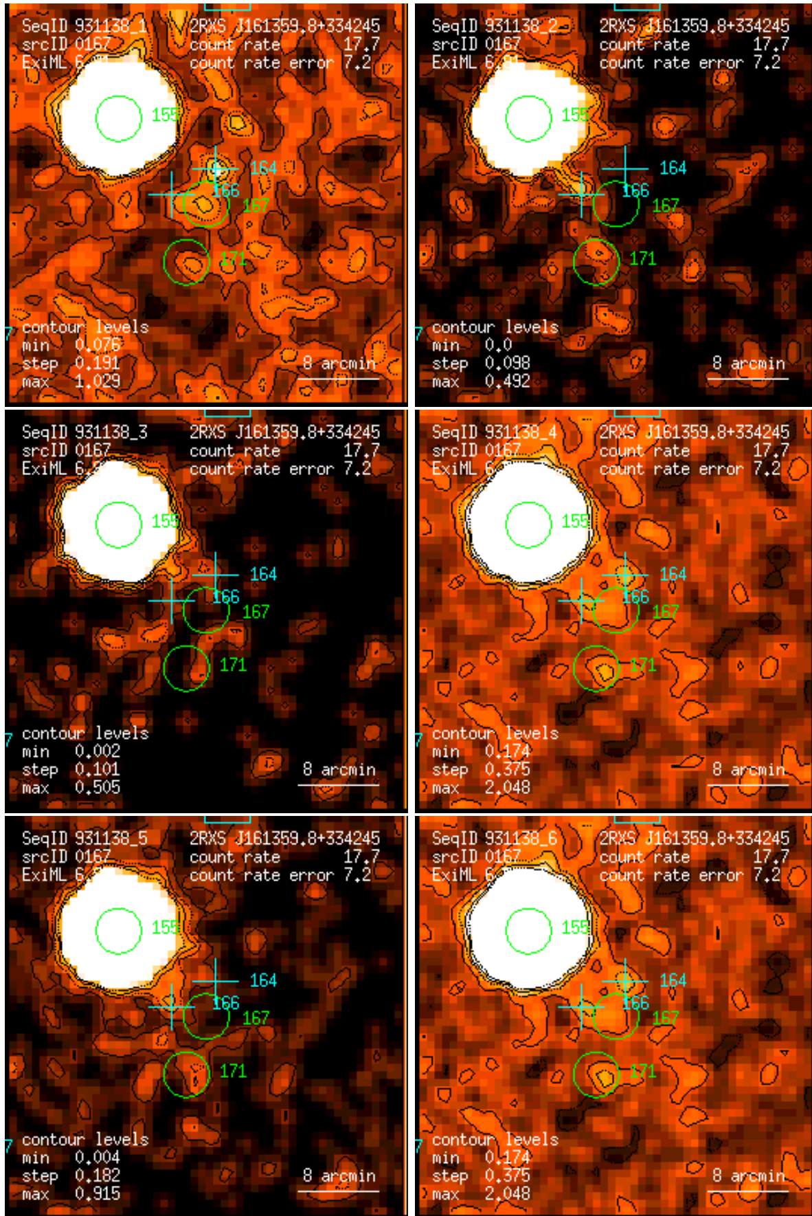
Figure 167: RASS 931138: detection 0167: band rate images, Gaussian filter: (1) PSPC channels 11 – 41, (2) 52 – 90, (3) 91 – 201, (4) 11 – 235, (5) 52 – 201, (6) 11 – 201. Broad band rates in counts/ks. Band rate contour levels in counts/ks/arcmin 2 .
