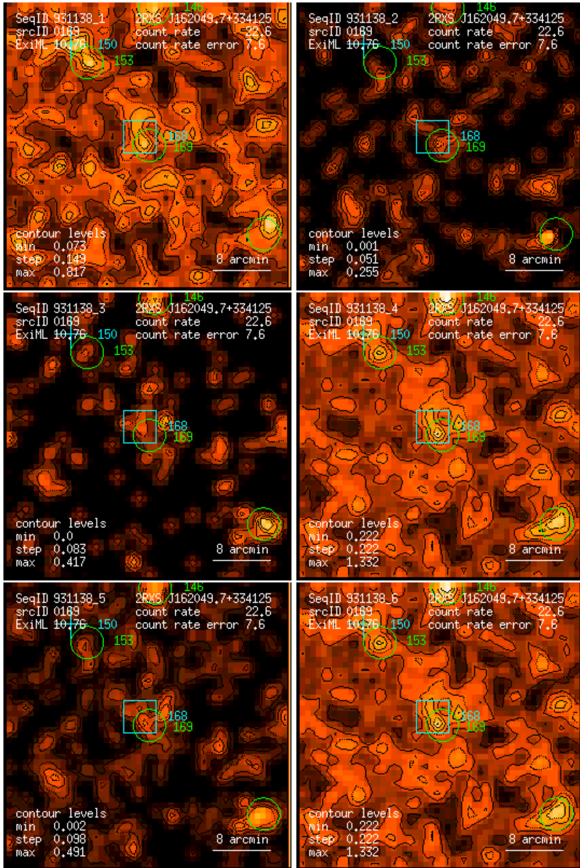
Figure 169: RASS 931138: detection 0169: band rate images, Gaussian filter: (1) PSPC channels 11 – 41, (2) 52 – 90, (3) 91 – 201, (4) 11 – 235, (5) 52 – 201, (6) 11 – 201. Broad band rates in counts/ks. Band rate contour levels in counts/ks/arcmin 2 .
