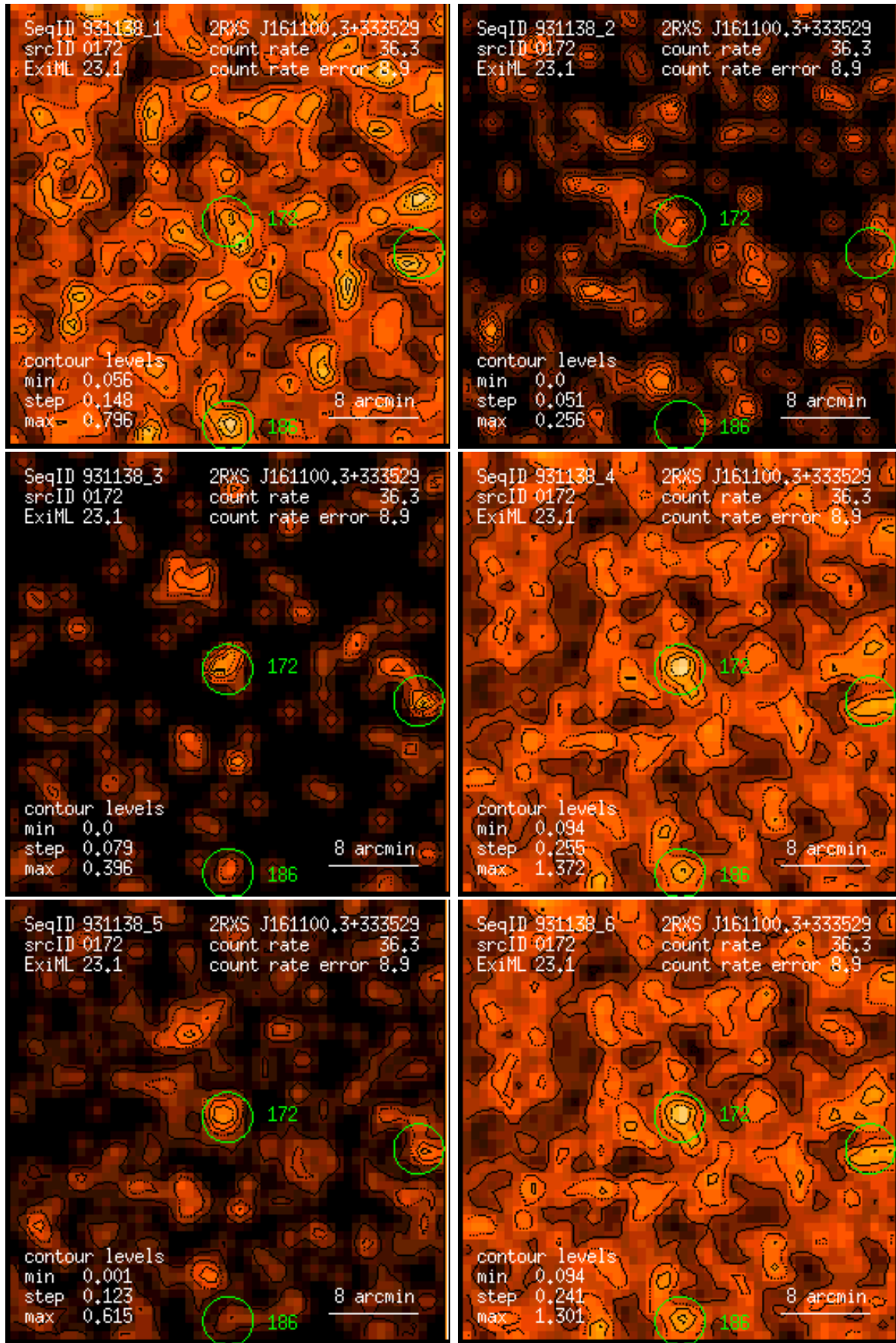
Figure 172: RASS 931138: detection 0172: band rate images, Gaussian filter: (1) PSPC channels 11 – 41, (2) 52 – 90, (3) 91 – 201, (4) 11 – 235, (5) 52 – 201, (6) 11 – 201. Broad band rates in counts/ks. Band rate contour levels in counts/ks/arcmin 2 .
