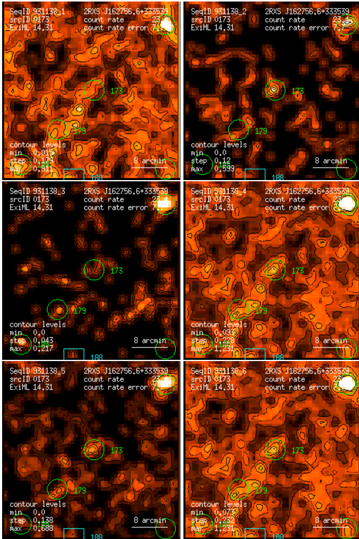
Figure 173: RASS 931138: detection 0173: band rate images, Gaussian filter: (1) PSPC channels 11 – 41, (2) 52 – 90, (3) 91 – 201, (4) 11 – 235, (5) 52 – 201, (6) 11 – 201. Broad band rates in counts/ks. Band rate contour levels in counts/ks/arcmin 2 .
