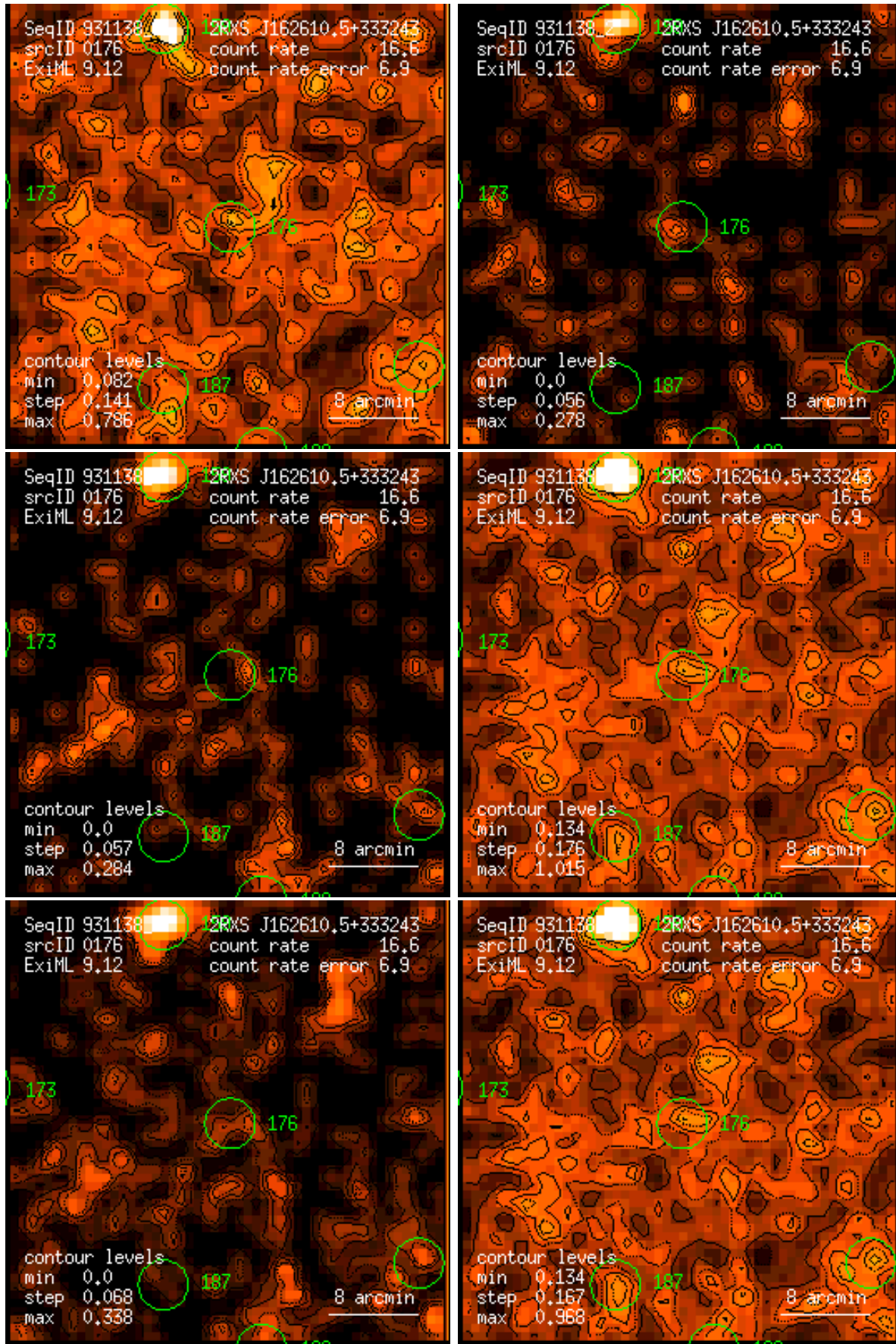
Figure 176: RASS 931138: detection 0176: band rate images, Gaussian filter: (1) PSPC channels 11 – 41, (2) 52 – 90, (3) 91 – 201, (4) 11 – 235, (5) 52 – 201, (6) 11 – 201. Broad band rates in counts/ks. Band rate contour levels in counts/ks/arcmin 2 .
