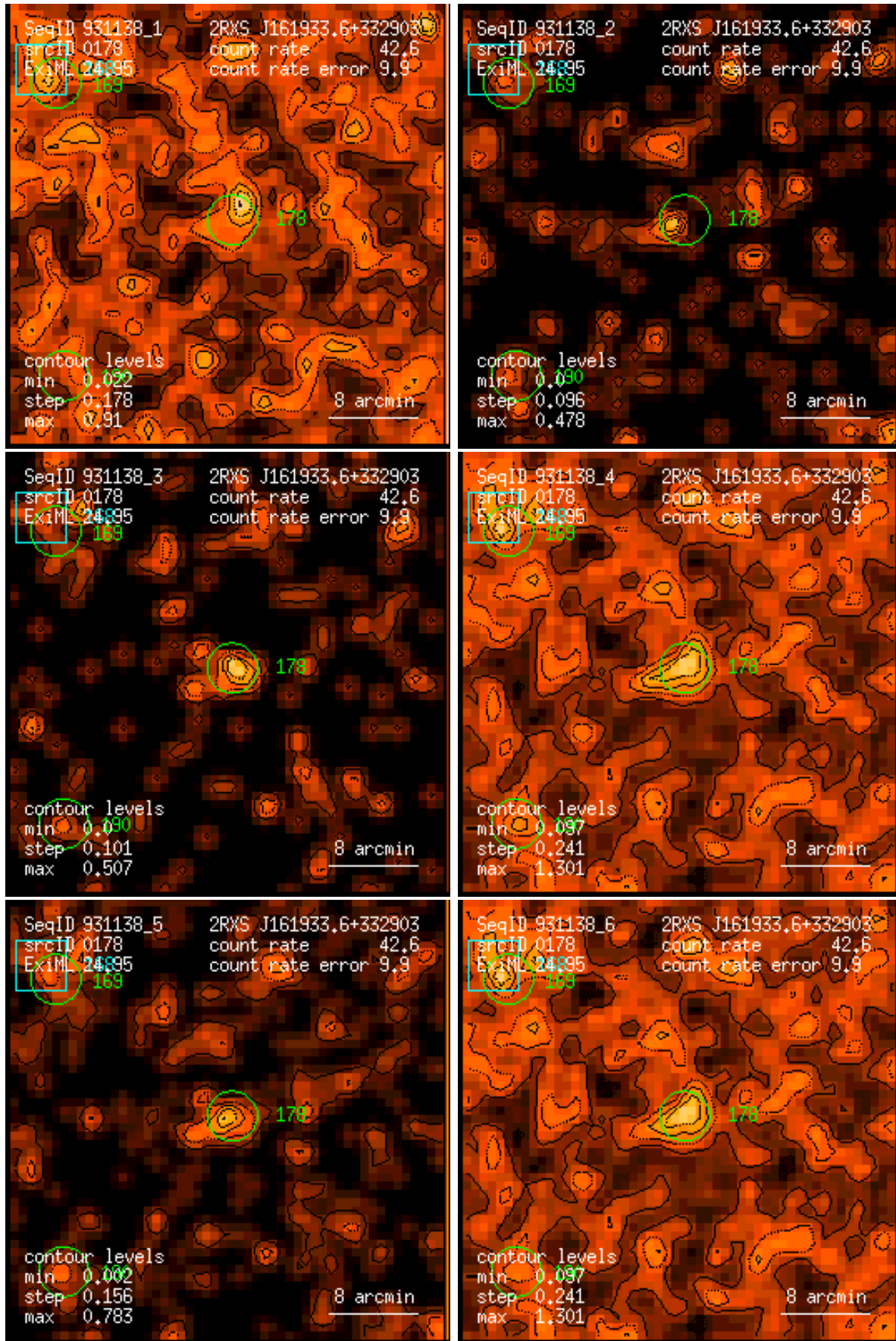
Figure 178: RASS 931138: detection 0178: band rate images, Gaussian filter: (1) PSPC channels 11 – 41, (2) 52 – 90, (3) 91 – 201, (4) 11 – 235, (5) 52 – 201, (6) 11 – 201. Broad band rates in counts/ks. Band rate contour levels in counts/ks/arcmin 2 .
