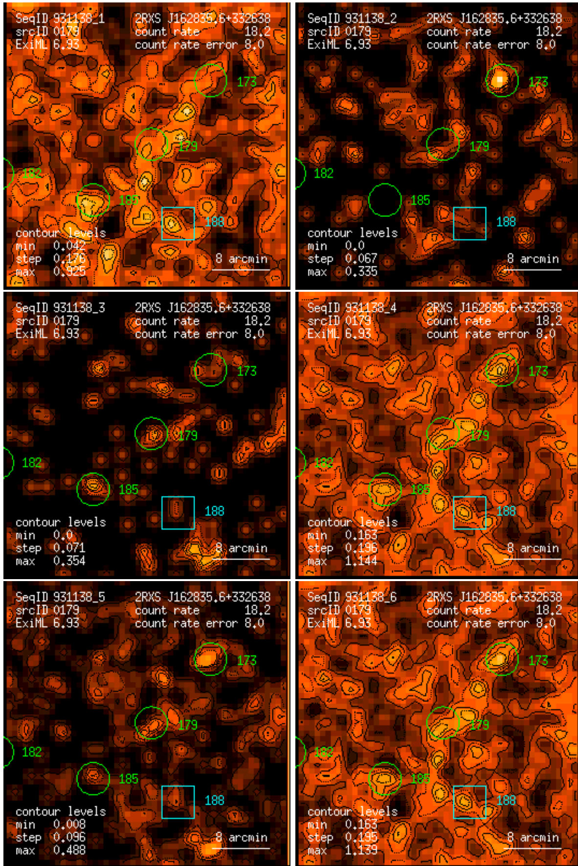
Figure 179: RASS 931138: detection 0179: band rate images, Gaussian filter: (1) PSPC channels 11 – 41, (2) 52 – 90, (3) 91 – 201, (4) 11 – 235, (5) 52 – 201, (6) 11 – 201. Broad band rates in counts/ks. Band rate contour levels in counts/ks/arcmin 2 .
