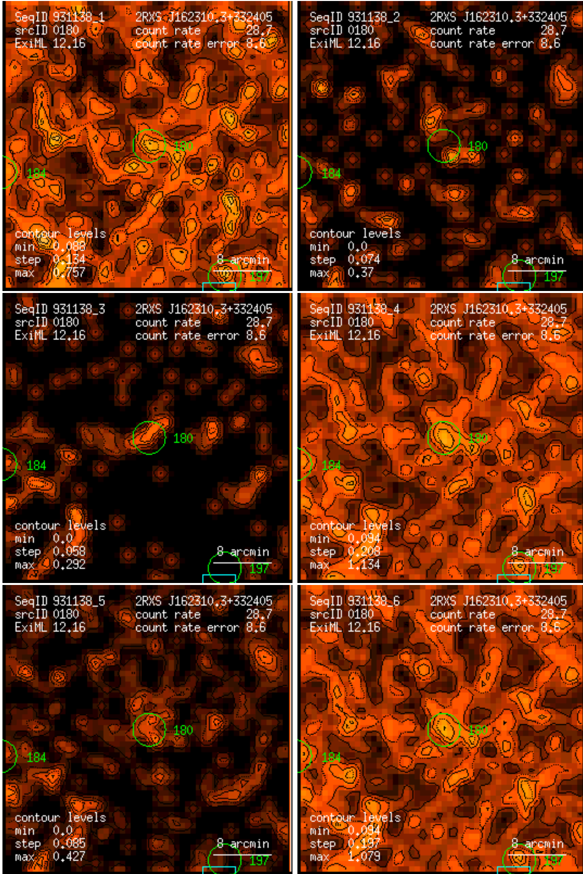
Figure 180: RASS 931138: detection 0180: band rate images, Gaussian filter: (1) PSPC channels 11 – 41, (2) 52 – 90, (3) 91 – 201, (4) 11 – 235, (5) 52 – 201, (6) 11 – 201. Broad band rates in counts/ks. Band rate contour levels in counts/ks/arcmin 2 .
