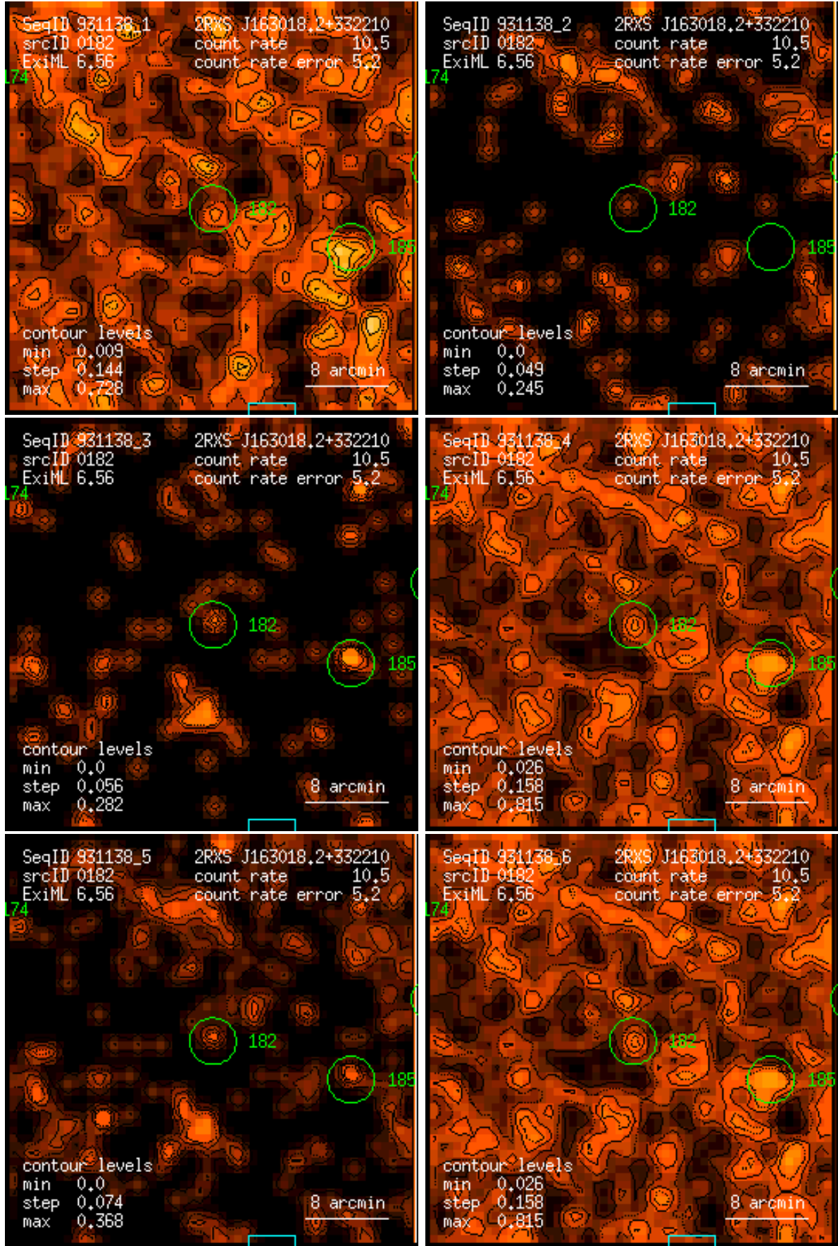
Figure 182: RASS 931138: detection 0182: band rate images, Gaussian filter: (1) PSPC channels 11 – 41, (2) 52 – 90, (3) 91 – 201, (4) 11 – 235, (5) 52 – 201, (6) 11 – 201. Broad band rates in counts/ks. Band rate contour levels in counts/ks/arcmin 2 .
