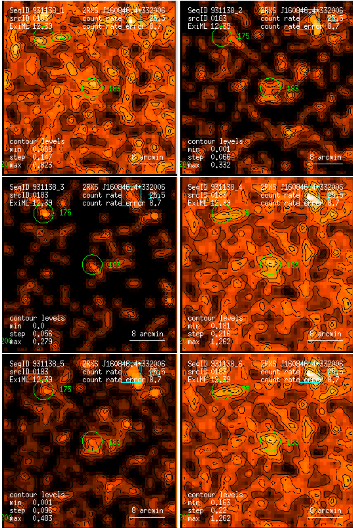
Figure 183: RASS 931138: detection 0183: band rate images, Gaussian filter: (1) PSPC channels 11 – 41, (2) 52 – 90, (3) 91 – 201, (4) 11 – 235, (5) 52 – 201, (6) 11 – 201. Broad band rates in counts/ks. Band rate contour levels in counts/ks/arcmin 2 .
