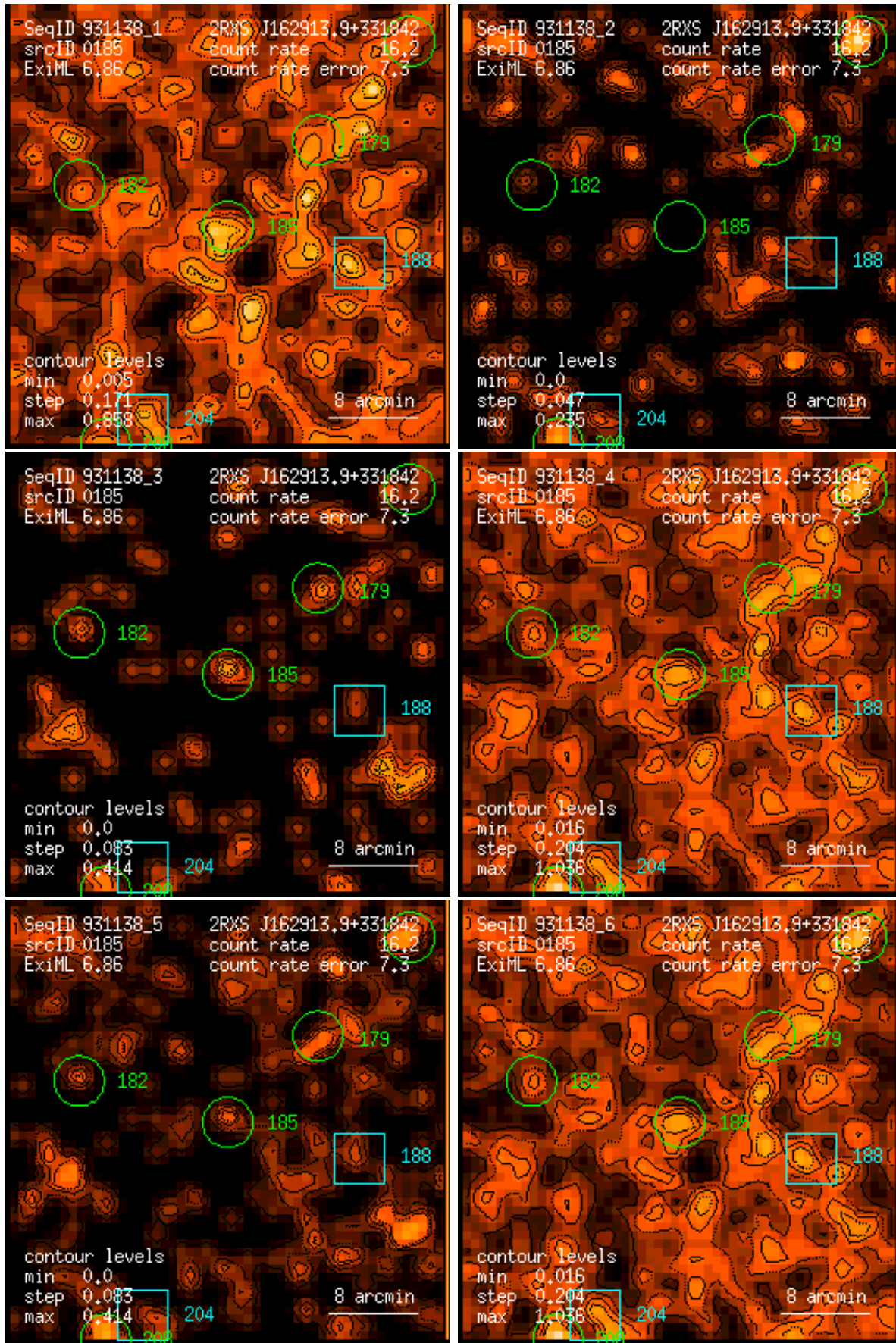
Figure 185: RASS 931138: detection 0185: band rate images, Gaussian filter: (1) PSPC channels 11 – 41, (2) 52 – 90, (3) 91 – 201, (4) 11 – 235, (5) 52 – 201, (6) 11 – 201. Broad band rates in counts/ks. Band rate contour levels in counts/ks/arcmin 2 .
