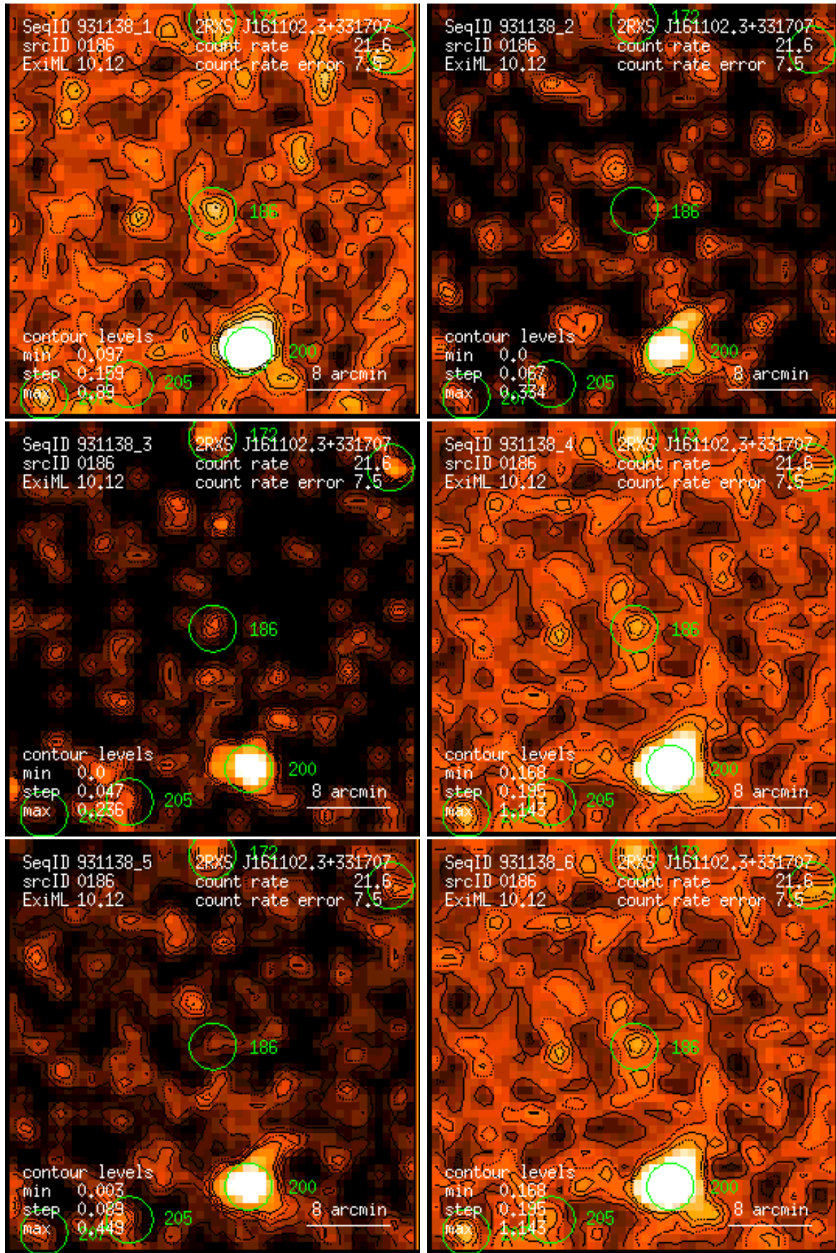
Figure 186: RASS 931138: detection 0186: band rate images, Gaussian filter: (1) PSPC channels 11 – 41, (2) 52 – 90, (3) 91 – 201, (4) 11 – 235, (5) 52 – 201, (6) 11 – 201. Broad band rates in counts/ks. Band rate contour levels in counts/ks/arcmin 2 .
