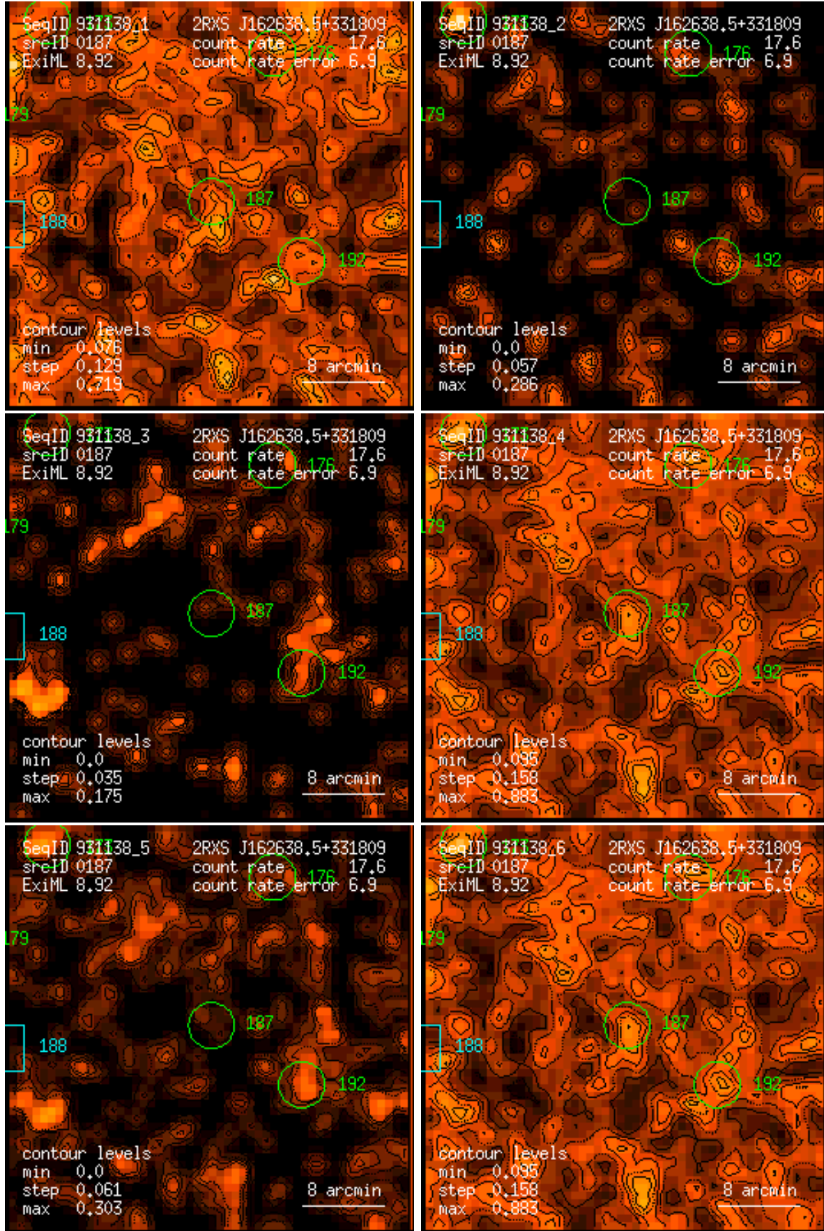
Figure 187: RASS 931138: detection 0187: band rate images, Gaussian filter: (1) PSPC channels 11 – 41, (2) 52 – 90, (3) 91 – 201, (4) 11 – 235, (5) 52 – 201, (6) 11 – 201. Broad band rates in counts/ks. Band rate contour levels in counts/ks/arcmin 2 .
