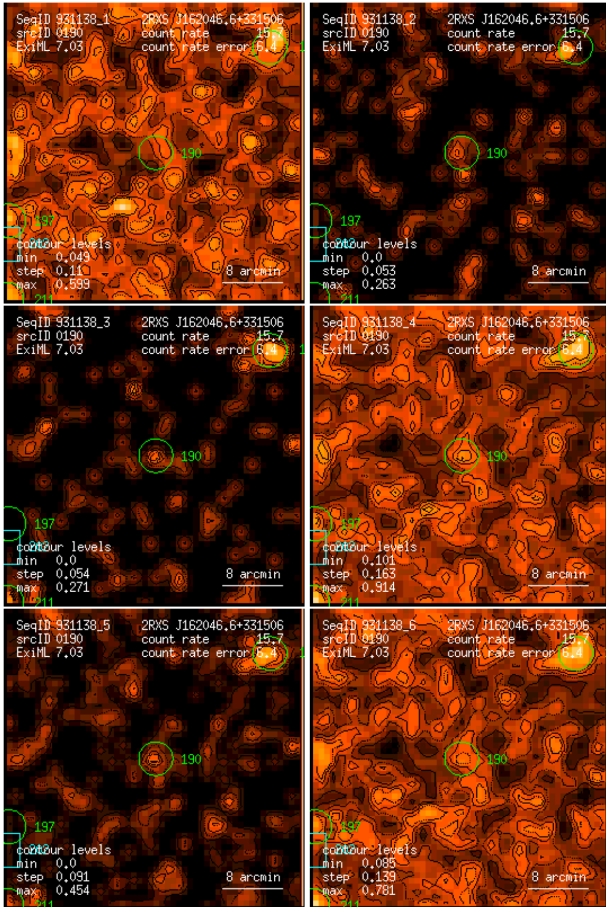
Figure 190: RASS 931138: detection 0190: band rate images, Gaussian filter: (1) PSPC channels 11 – 41, (2) 52 – 90, (3) 91 – 201, (4) 11 – 235, (5) 52 – 201, (6) 11 – 201. Broad band rates in counts/ks. Band rate contour levels in counts/ks/arcmin 2 .
