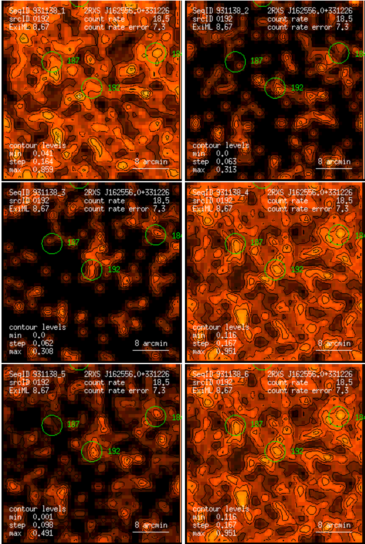
Figure 192: RASS 931138: detection 0192: band rate images, Gaussian filter: (1) PSPC channels 11 – 41, (2) 52 – 90, (3) 91 – 201, (4) 11 – 235, (5) 52 – 201, (6) 11 – 201. Broad band rates in counts/ks. Band rate contour levels in counts/ks/arcmin 2 .
