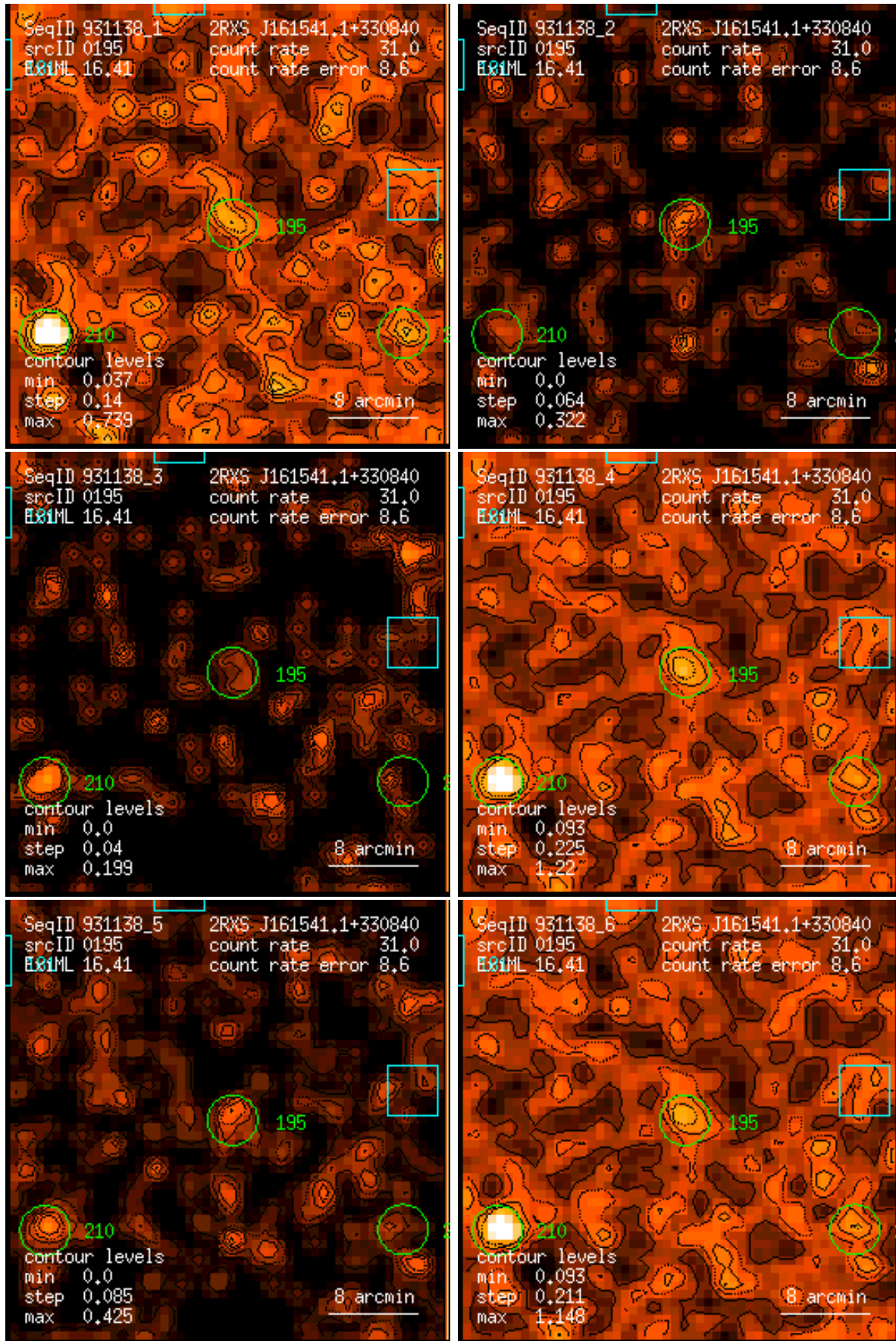
Figure 195: RASS 931138: detection 0195: band rate images, Gaussian filter: (1) PSPC channels 11 – 41, (2) 52 – 90, (3) 91 – 201, (4) 11 – 235, (5) 52 – 201, (6) 11 – 201. Broad band rates in counts/ks. Band rate contour levels in counts/ks/arcmin 2 .
