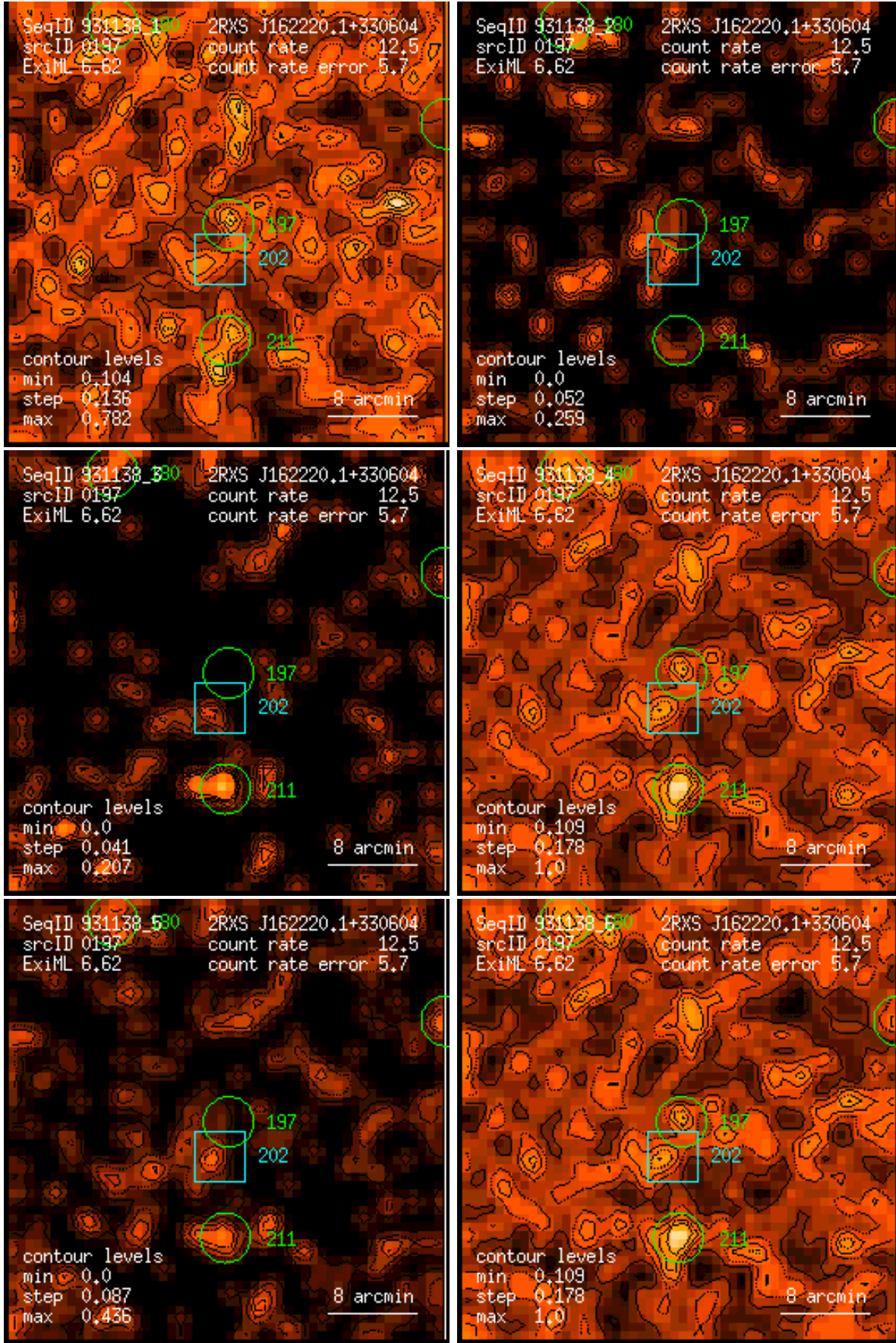
Figure 197: RASS 931138: detection 0197: band rate images, Gaussian filter: (1) PSPC channels 11 – 41, (2) 52 – 90, (3) 91 – 201, (4) 11 – 235, (5) 52 – 201, (6) 11 – 201. Broad band rates in counts/ks. Band rate contour levels in counts/ks/arcmin 2 .
