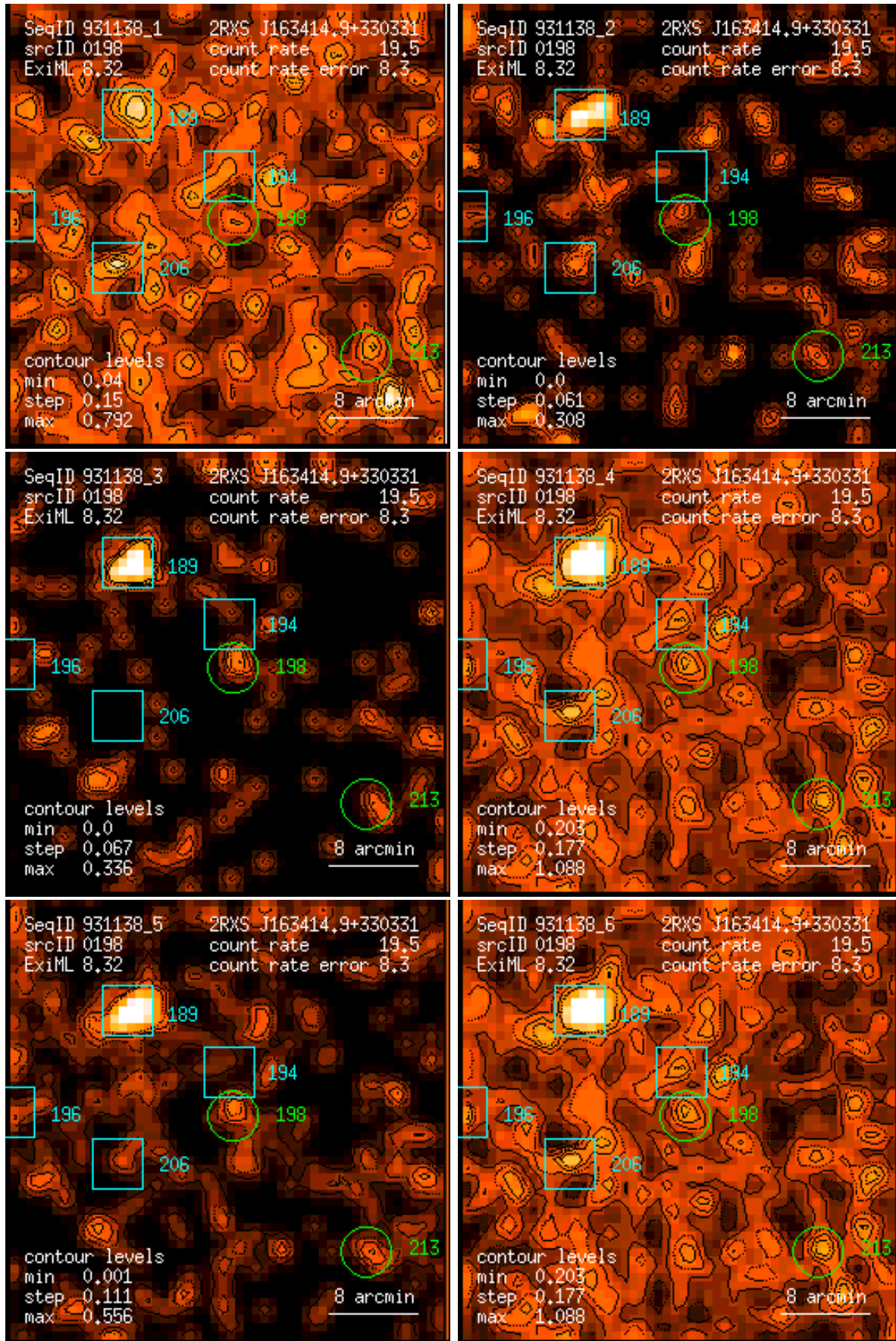
Figure 198: RASS 931138: detection 0198: band rate images, Gaussian filter: (1) PSPC channels 11 – 41, (2) 52 – 90, (3) 91 – 201, (4) 11 – 235, (5) 52 – 201, (6) 11 – 201. Broad band rates in counts/ks. Band rate contour levels in counts/ks/arcmin 2 .
