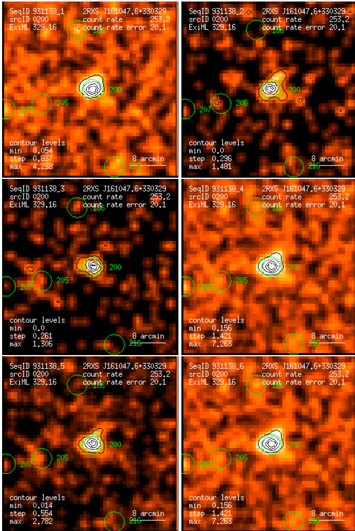
Figure 200: RASS 931138: detection 0200: band rate images, Gaussian filter: (1) PSPC channels 11 – 41, (2) 52 – 90, (3) 91 – 201, (4) 11 – 235, (5) 52 – 201, (6) 11 – 201. Broad band rates in counts/ks. Band rate contour levels in counts/ks/arcmin 2 .
