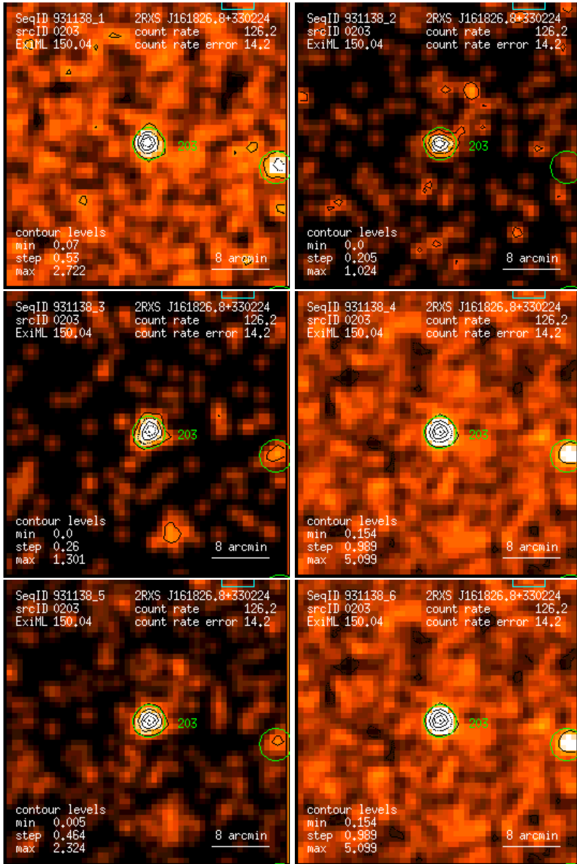
Figure 203: RASS 931138: detection 0203: band rate images, Gaussian filter: (1) PSPC channels 11 – 41, (2) 52 – 90, (3) 91 – 201, (4) 11 – 235, (5) 52 – 201, (6) 11 – 201. Broad band rates in counts/ks. Band rate contour levels in counts/ks/arcmin 2 .
