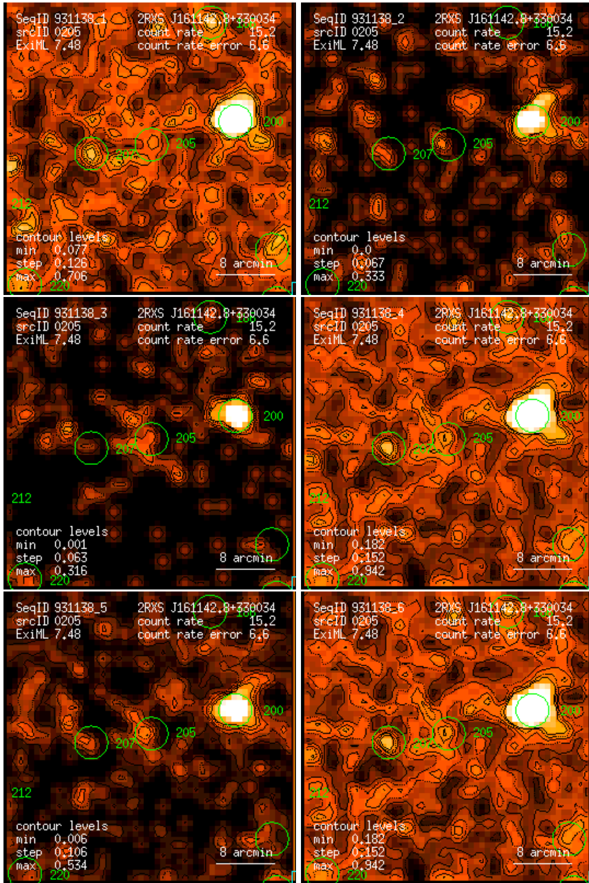
Figure 205: RASS 931138: detection 0205: band rate images, Gaussian filter: (1) PSPC channels 11 – 41, (2) 52 – 90, (3) 91 – 201, (4) 11 – 235, (5) 52 – 201, (6) 11 – 201. Broad band rates in counts/ks. Band rate contour levels in counts/ks/arcmin 2 .
