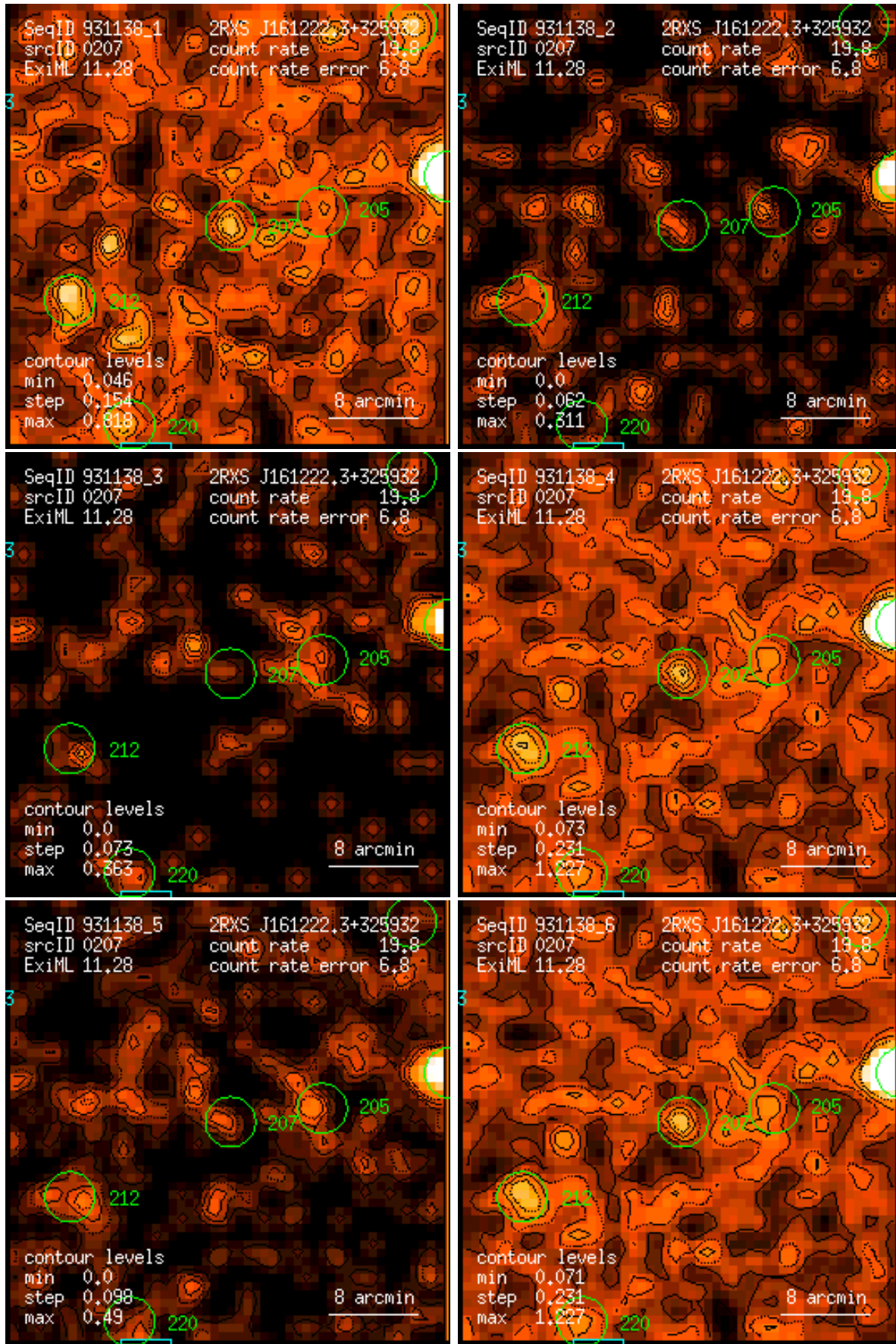
Figure 207: RASS 931138: detection 0207: band rate images, Gaussian filter: (1) PSPC channels 11 – 41, (2) 52 – 90, (3) 91 – 201, (4) 11 – 235, (5) 52 – 201, (6) 11 – 201. Broad band rates in counts/ks. Band rate contour levels in counts/ks/arcmin 2 .
