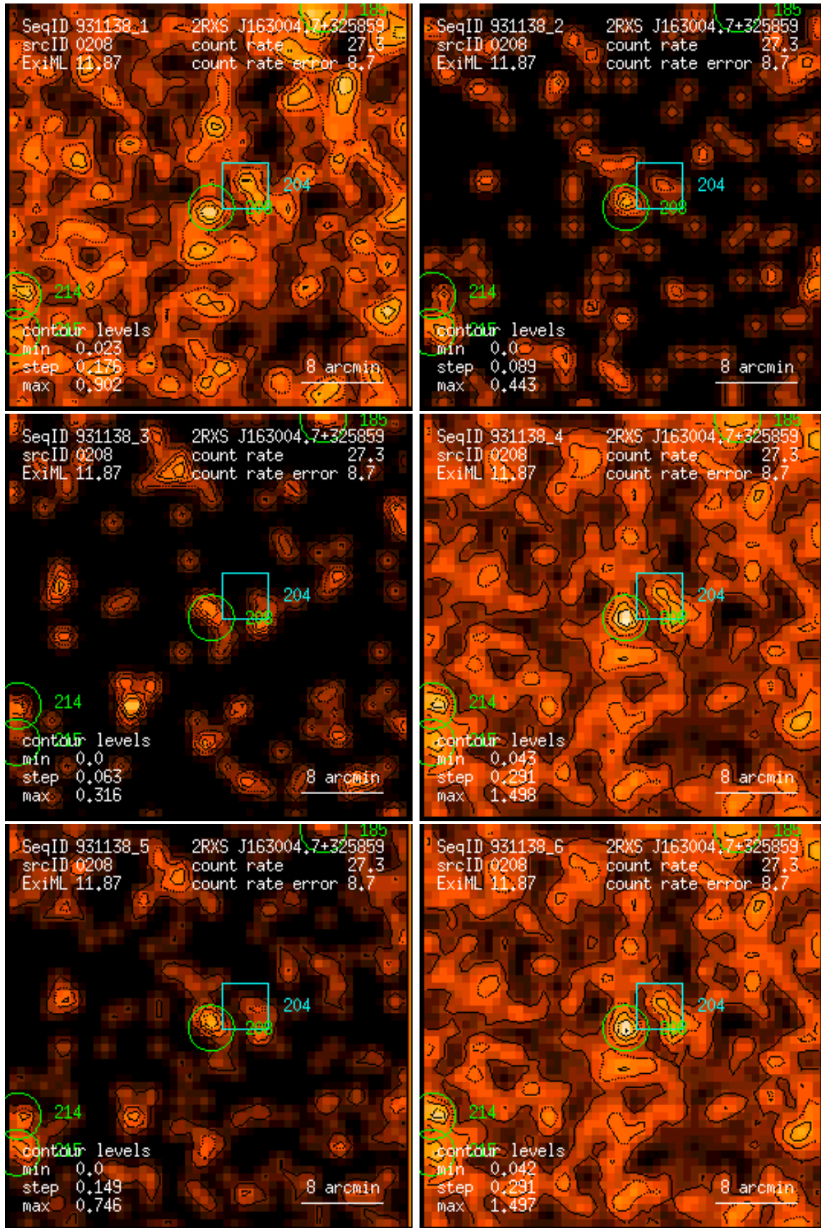
Figure 208: RASS 931138: detection 0208: band rate images, Gaussian filter: (1) PSPC channels 11 – 41, (2) 52 – 90, (3) 91 – 201, (4) 11 – 235, (5) 52 – 201, (6) 11 – 201. Broad band rates in counts/ks. Band rate contour levels in counts/ks/arcmin 2 .
