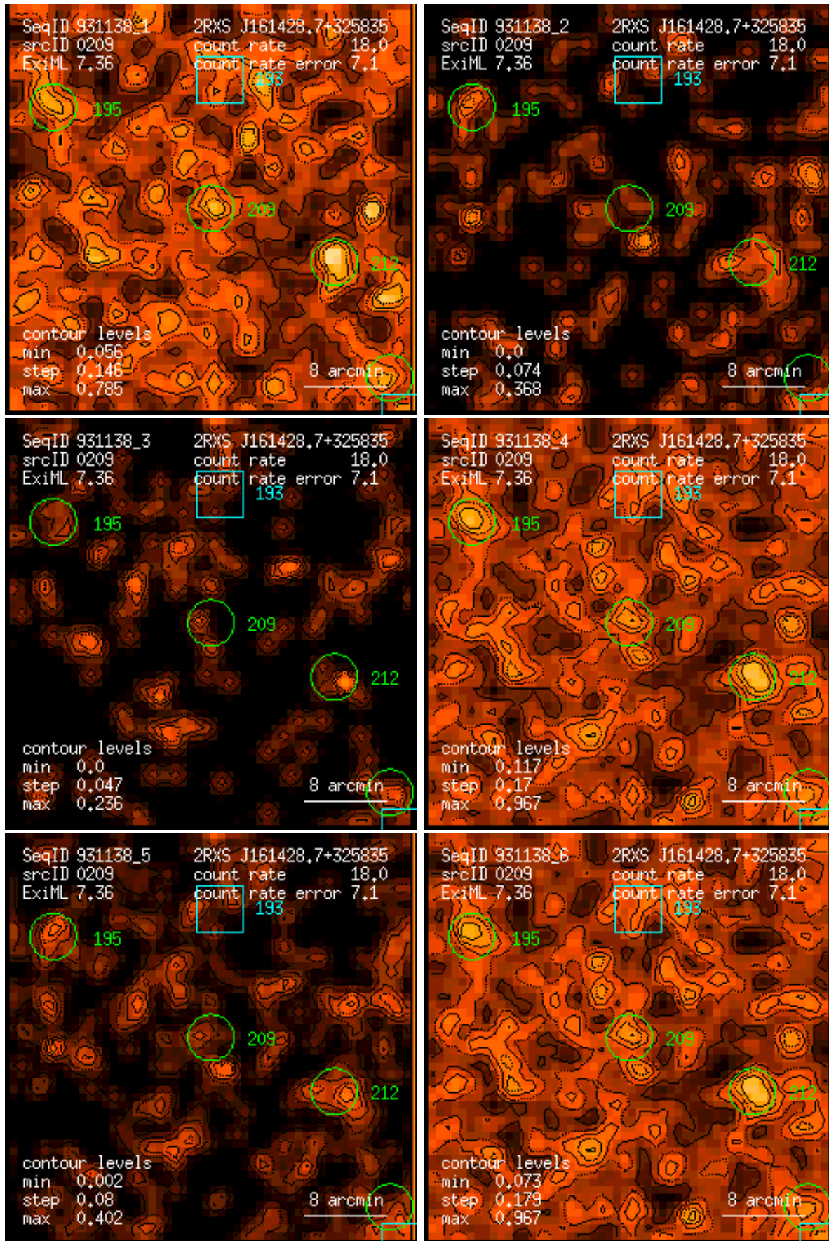
Figure 209: RASS 931138: detection 0209: band rate images, Gaussian filter: (1) PSPC channels 11 – 41, (2) 52 – 90, (3) 91 – 201, (4) 11 – 235, (5) 52 – 201, (6) 11 – 201. Broad band rates in counts/ks. Band rate contour levels in counts/ks/arcmin 2 .
