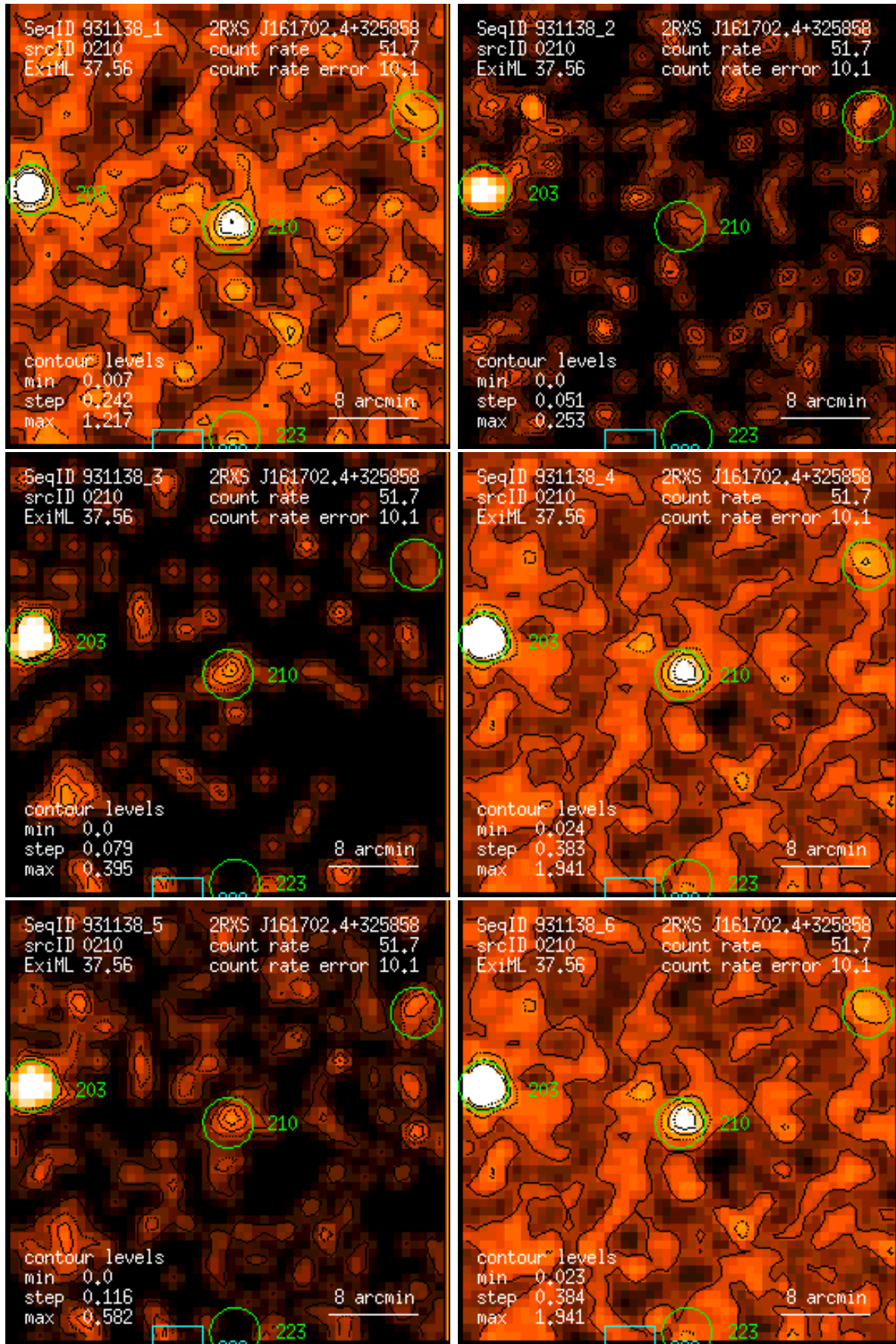
Figure 210: RASS 931138: detection 0210: band rate images, Gaussian filter: (1) PSPC channels 11 – 41, (2) 52 – 90, (3) 91 – 201, (4) 11 – 235, (5) 52 – 201, (6) 11 – 201. Broad band rates in counts/ks. Band rate contour levels in counts/ks/arcmin 2 .
