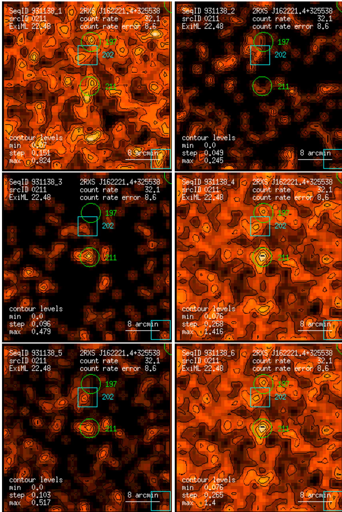
Figure 211: RASS 931138: detection 0211: band rate images, Gaussian filter: (1) PSPC channels 11 – 41, (2) 52 – 90, (3) 91 – 201, (4) 11 – 235, (5) 52 – 201, (6) 11 – 201. Broad band rates in counts/ks. Band rate contour levels in counts/ks/arcmin 2 .
