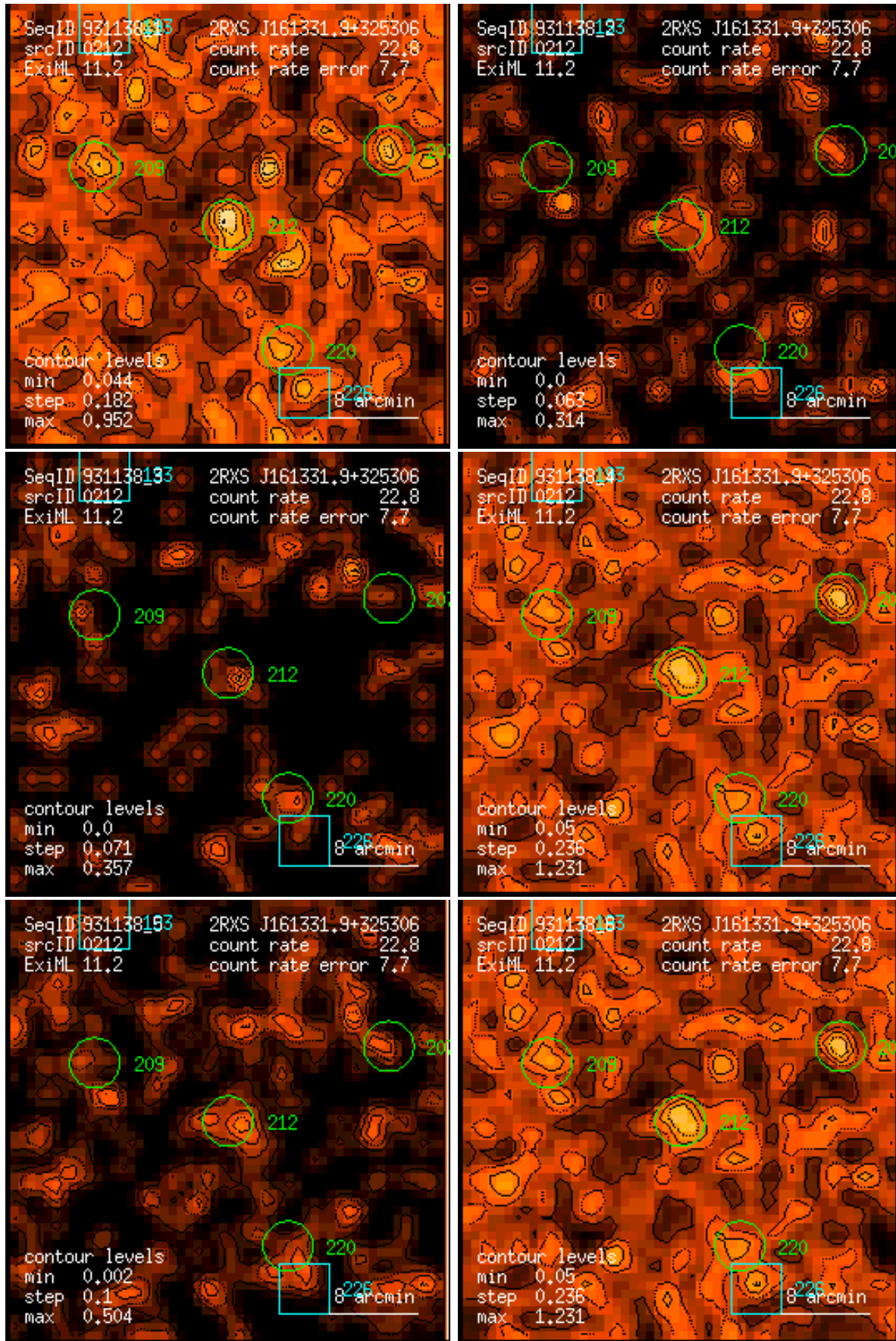
Figure 212: RASS 931138: detection 0212: band rate images, Gaussian filter: (1) PSPC channels 11 – 41, (2) 52 – 90, (3) 91 – 201, (4) 11 – 235, (5) 52 – 201, (6) 11 – 201. Broad band rates in counts/ks. Band rate contour levels in counts/ks/arcmin 2 .
