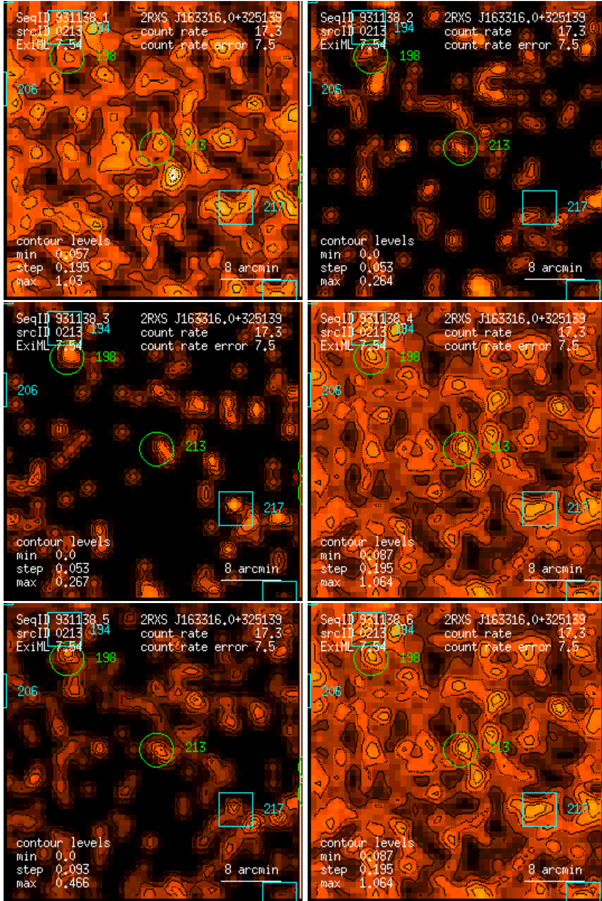
Figure 213: RASS 931138: detection 0213: band rate images, Gaussian filter: (1) PSPC channels 11 – 41, (2) 52 – 90, (3) 91 – 201, (4) 11 – 235, (5) 52 – 201, (6) 11 – 201. Broad band rates in counts/ks. Band rate contour levels in counts/ks/arcmin 2 .
