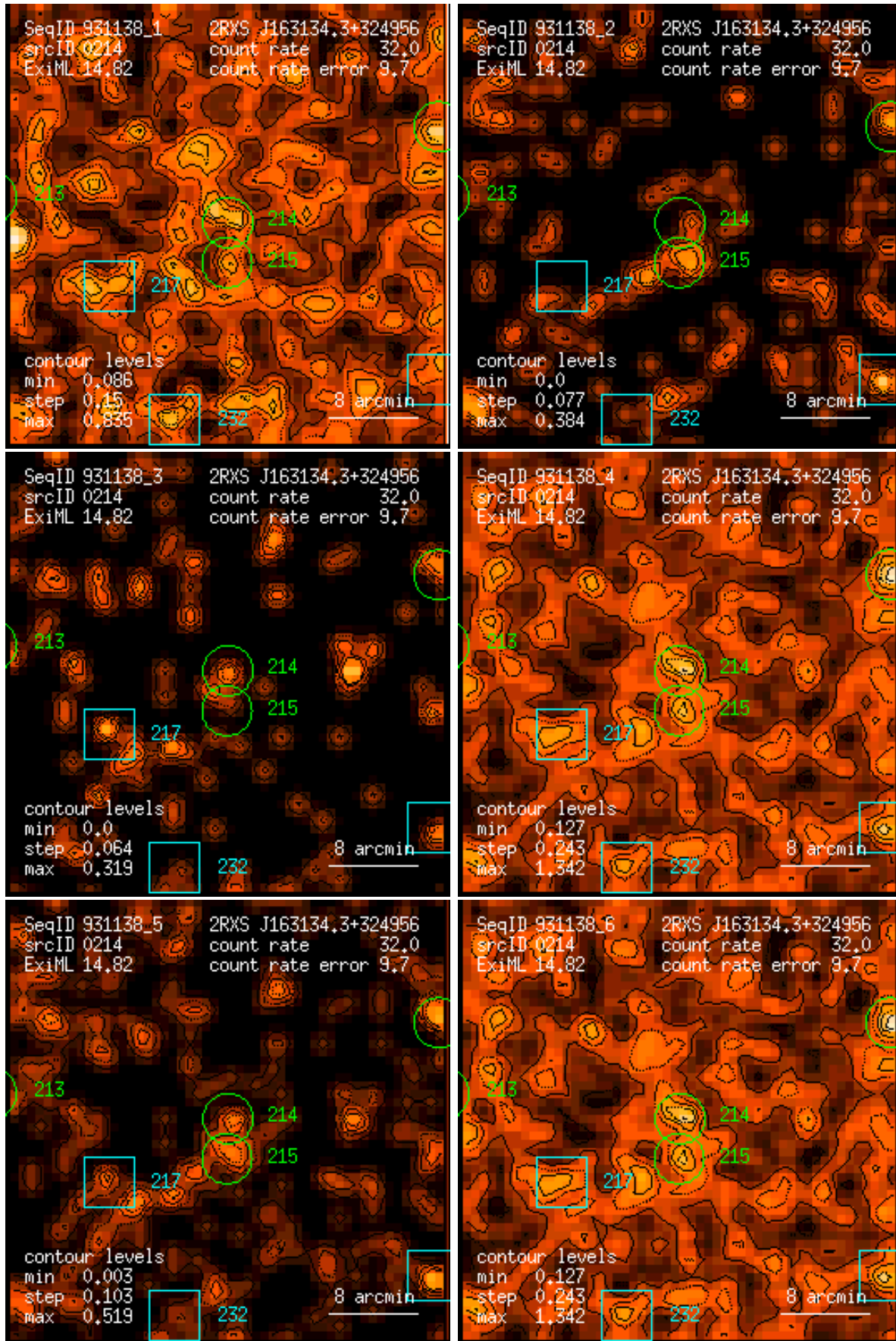
Figure 214: RASS 931138: detection 0214: band rate images, Gaussian filter: (1) PSPC channels 11 – 41, (2) 52 – 90, (3) 91 – 201, (4) 11 – 235, (5) 52 – 201, (6) 11 – 201. Broad band rates in counts/ks. Band rate contour levels in counts/ks/arcmin 2 .
