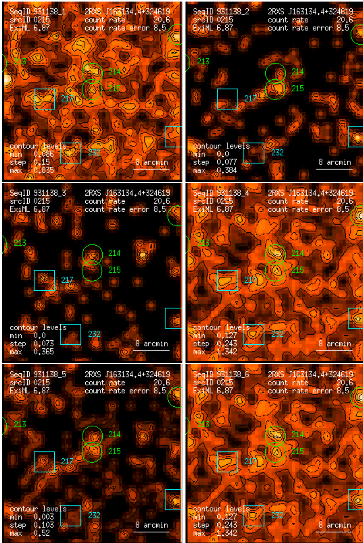
Figure 215: RASS 931138: detection 0215: band rate images, Gaussian filter: (1) PSPC channels 11 – 41, (2) 52 – 90, (3) 91 – 201, (4) 11 – 235, (5) 52 – 201, (6) 11 – 201. Broad band rates in counts/ks. Band rate contour levels in counts/ks/arcmin 2 .
