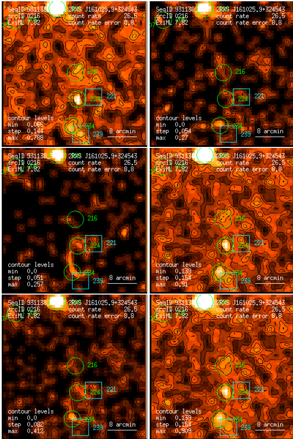
Figure 216: RASS 931138: detection 0216: band rate images, Gaussian filter: (1) PSPC channels 11 – 41, (2) 52 – 90, (3) 91 – 201, (4) 11 – 235, (5) 52 – 201, (6) 11 – 201. Broad band rates in counts/ks. Band rate contour levels in counts/ks/arcmin 2 .
