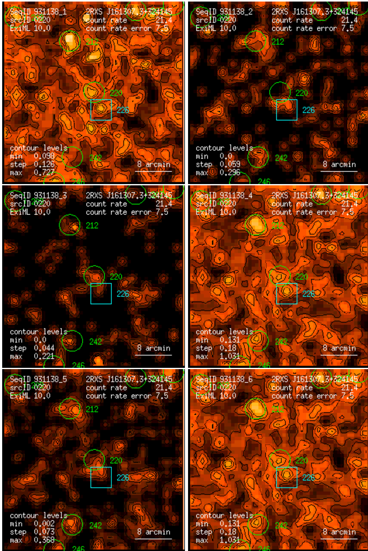
Figure 220: RASS 931138: detection 0220: band rate images, Gaussian filter: (1) PSPC channels 11 – 41, (2) 52 – 90, (3) 91 – 201, (4) 11 – 235, (5) 52 – 201, (6) 11 – 201. Broad band rates in counts/ks. Band rate contour levels in counts/ks/arcmin 2 .
