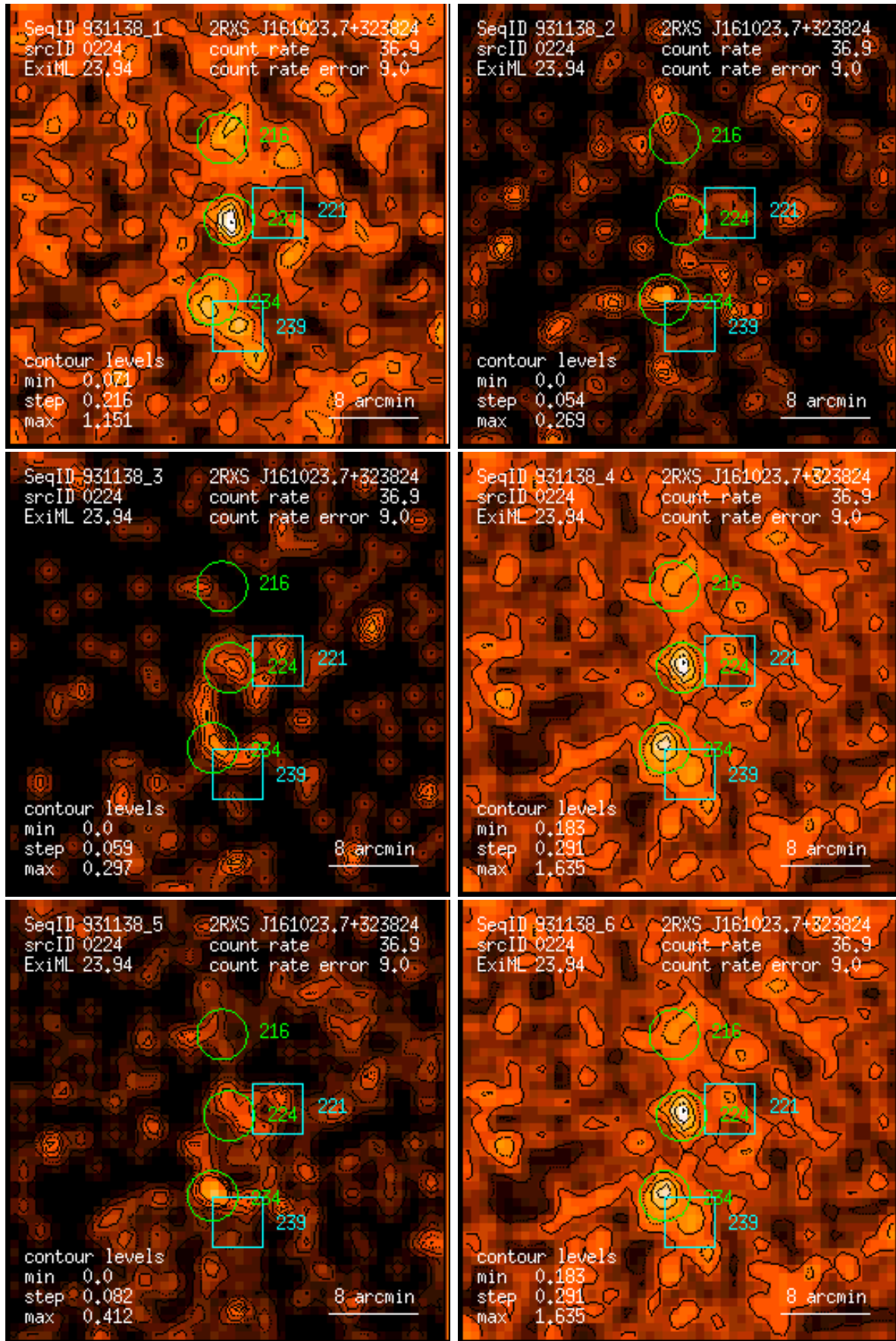
Figure 224: RASS 931138: detection 0224: band rate images, Gaussian filter: (1) PSPC channels 11 – 41, (2) 52 – 90, (3) 91 – 201, (4) 11 – 235, (5) 52 – 201, (6) 11 – 201. Broad band rates in counts/ks. Band rate contour levels in counts/ks/arcmin 2 .
