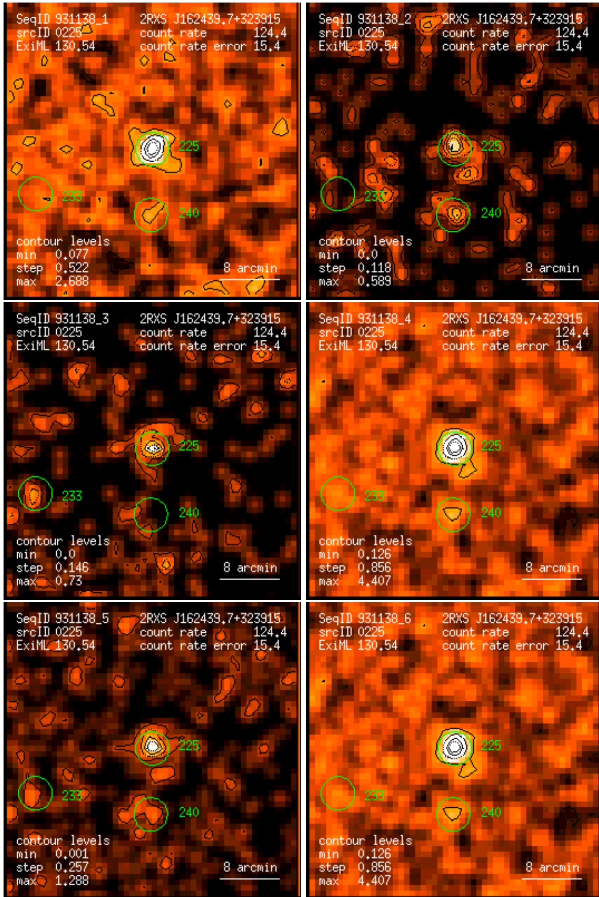
Figure 225: RASS 931138: detection 0225: band rate images, Gaussian filter: (1) PSPC channels 11 – 41, (2) 52 – 90, (3) 91 – 201, (4) 11 – 235, (5) 52 – 201, (6) 11 – 201. Broad band rates in counts/ks. Band rate contour levels in counts/ks/arcmin 2 .
