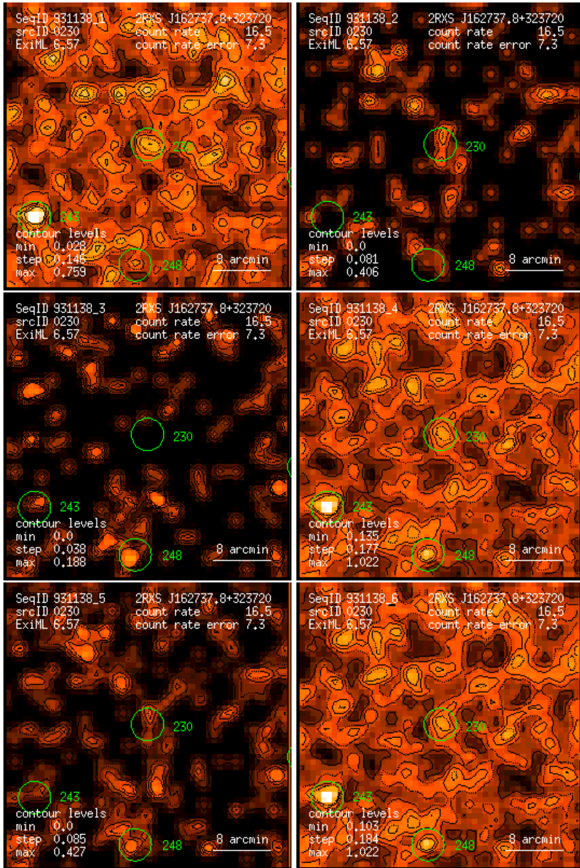
Figure 230: RASS 931138: detection 0230: band rate images, Gaussian filter: (1) PSPC channels 11 – 41, (2) 52 – 90, (3) 91 – 201, (4) 11 – 235, (5) 52 – 201, (6) 11 – 201. Broad band rates in counts/ks. Band rate contour levels in counts/ks/arcmin 2 .
