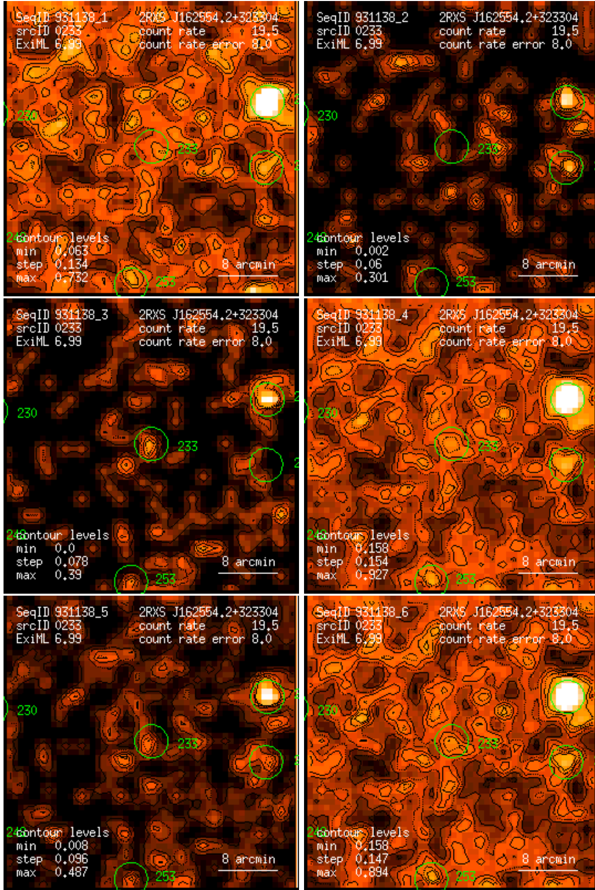
Figure 233: RASS 931138: detection 0233: band rate images, Gaussian filter: (1) PSPC channels 11 – 41, (2) 52 – 90, (3) 91 – 201, (4) 11 – 235, (5) 52 – 201, (6) 11 – 201. Broad band rates in counts/ks. Band rate contour levels in counts/ks/arcmin 2 .
