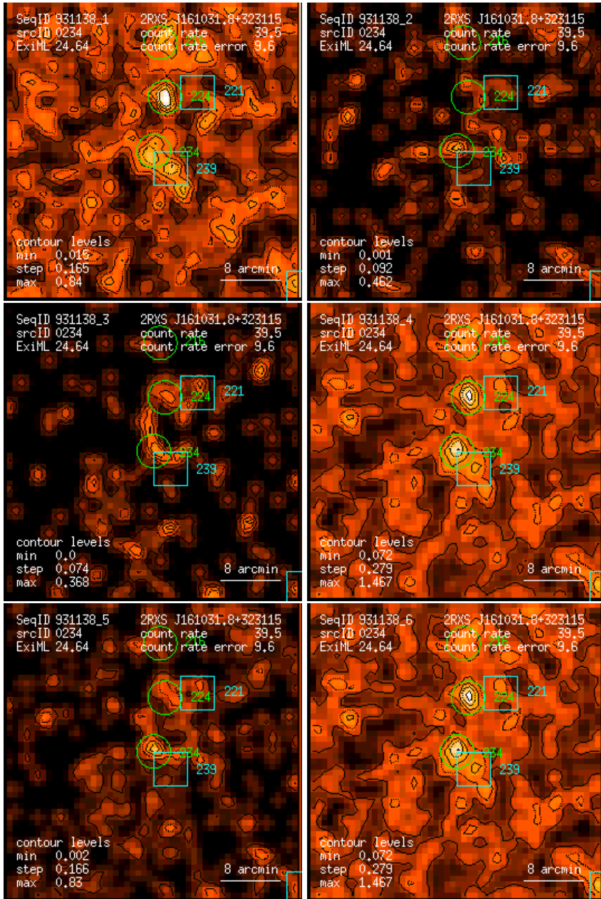
Figure 234: RASS 931138: detection 0234: band rate images, Gaussian filter: (1) PSPC channels 11 – 41, (2) 52 – 90, (3) 91 – 201, (4) 11 – 235, (5) 52 – 201, (6) 11 – 201. Broad band rates in counts/ks. Band rate contour levels in counts/ks/arcmin 2 .
