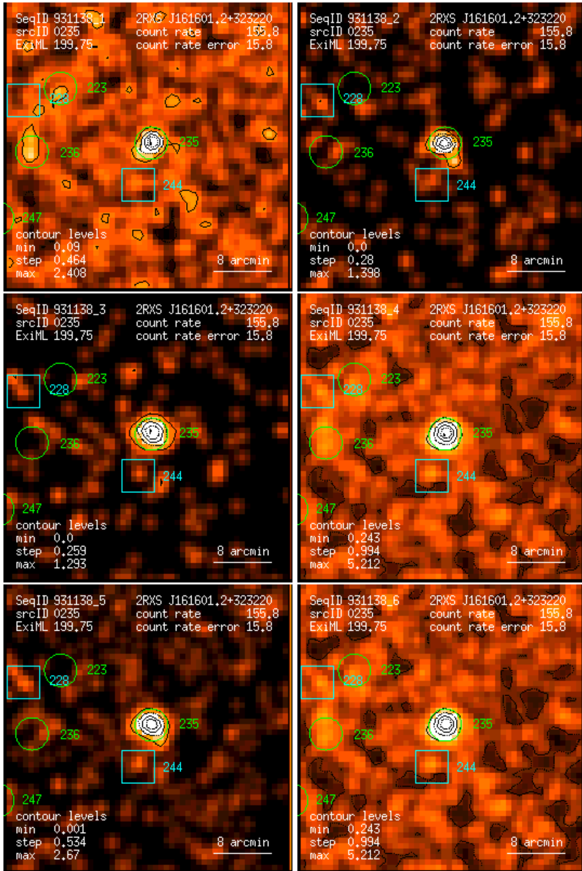
Figure 235: RASS 931138: detection 0235: band rate images, Gaussian filter: (1) PSPC channels 11 – 41, (2) 52 – 90, (3) 91 – 201, (4) 11 – 235, (5) 52 – 201, (6) 11 – 201. Broad band rates in counts/ks. Band rate contour levels in counts/ks/arcmin 2 .
