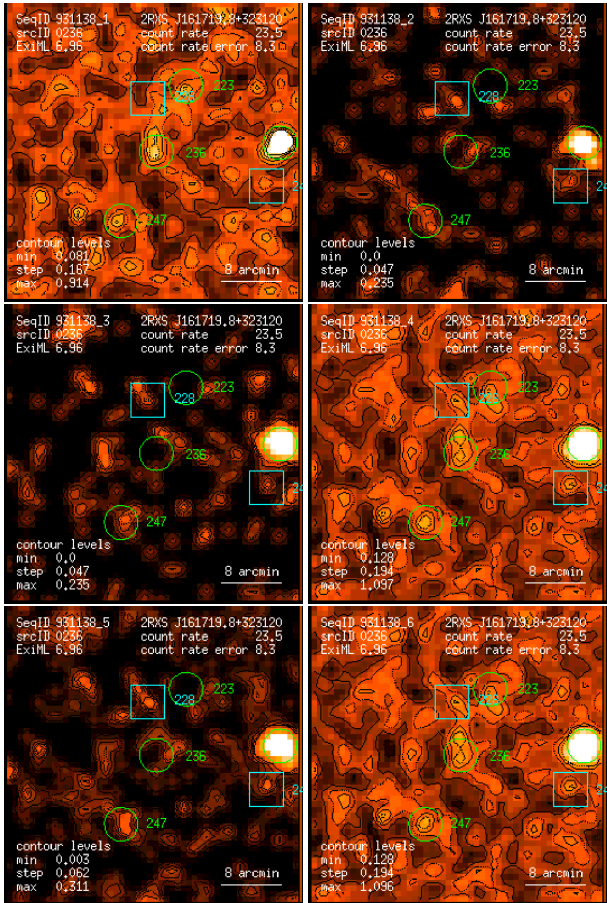
Figure 236: RASS 931138: detection 0236: band rate images, Gaussian filter: (1) PSPC channels 11 – 41, (2) 52 – 90, (3) 91 – 201, (4) 11 – 235, (5) 52 – 201, (6) 11 – 201. Broad band rates in counts/ks. Band rate contour levels in counts/ks/arcmin 2 .
