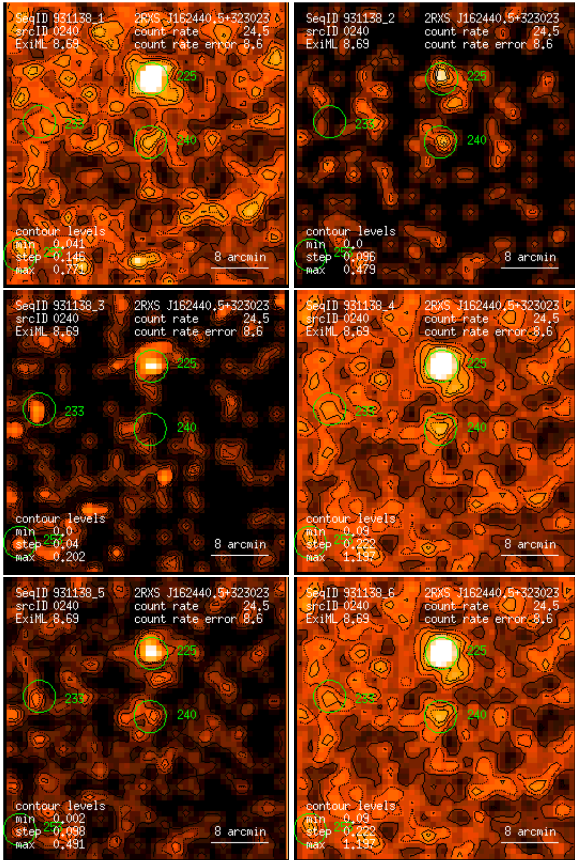
Figure 240: RASS 931138: detection 0240: band rate images, Gaussian filter: (1) PSPC channels 11 – 41, (2) 52 – 90, (3) 91 – 201, (4) 11 – 235, (5) 52 – 201, (6) 11 – 201. Broad band rates in counts/ks. Band rate contour levels in counts/ks/arcmin 2 .
