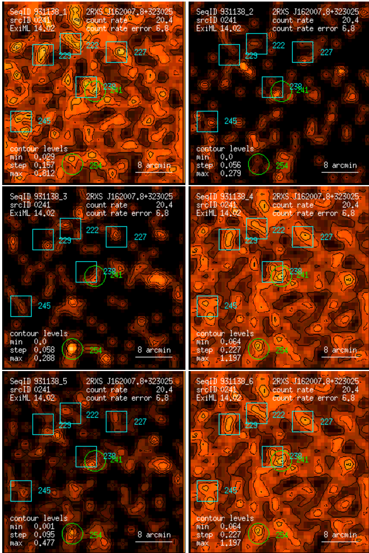
Figure 241: RASS 931138: detection 0241: band rate images, Gaussian filter: (1) PSPC channels 11 – 41, (2) 52 – 90, (3) 91 – 201, (4) 11 – 235, (5) 52 – 201, (6) 11 – 201. Broad band rates in counts/ks. Band rate contour levels in counts/ks/arcmin 2 .
