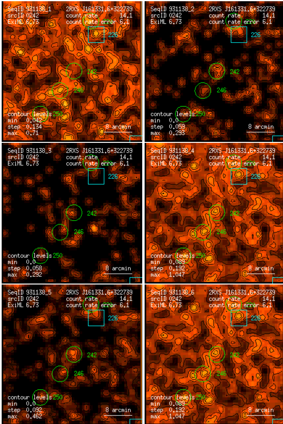
Figure 242: RASS 931138: detection 0242: band rate images, Gaussian filter: (1) PSPC channels 11 – 41, (2) 52 – 90, (3) 91 – 201, (4) 11 – 235, (5) 52 – 201, (6) 11 – 201. Broad band rates in counts/ks. Band rate contour levels in counts/ks/arcmin 2 .
