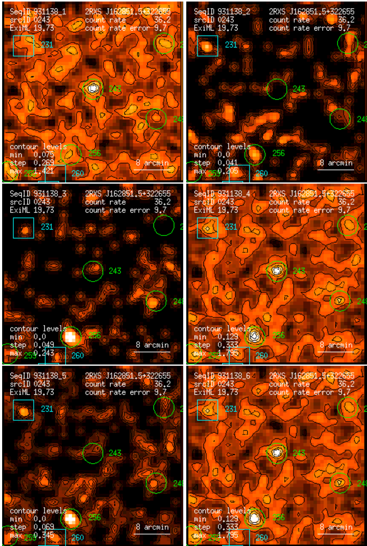
Figure 243: RASS 931138: detection 0243: band rate images, Gaussian filter: (1) PSPC channels 11 – 41, (2) 52 – 90, (3) 91 – 201, (4) 11 – 235, (5) 52 – 201, (6) 11 – 201. Broad band rates in counts/ks. Band rate contour levels in counts/ks/arcmin 2 .
