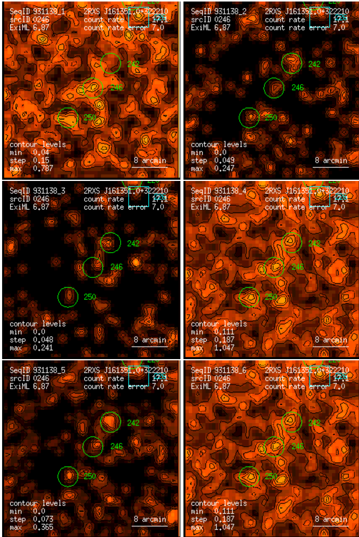
Figure 246: RASS 931138: detection 0246: band rate images, Gaussian filter: (1) PSPC channels 11 – 41, (2) 52 – 90, (3) 91 – 201, (4) 11 – 235, (5) 52 – 201, (6) 11 – 201. Broad band rates in counts/ks. Band rate contour levels in counts/ks/arcmin 2 .
