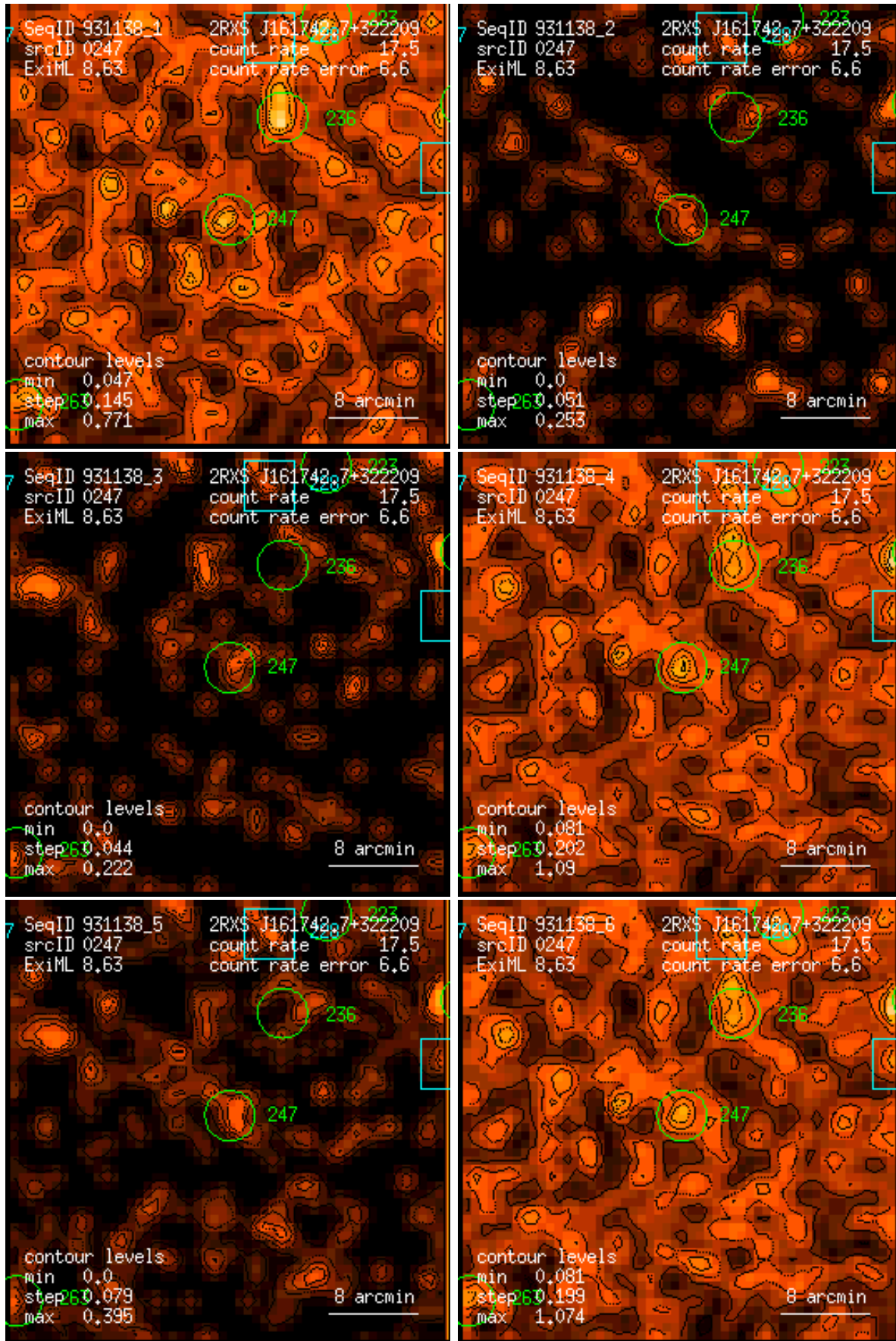
Figure 247: RASS 931138: detection 0247: band rate images, Gaussian filter: (1) PSPC channels 11 – 41, (2) 52 – 90, (3) 91 – 201, (4) 11 – 235, (5) 52 – 201, (6) 11 – 201. Broad band rates in counts/ks. Band rate contour levels in counts/ks/arcmin 2 .
