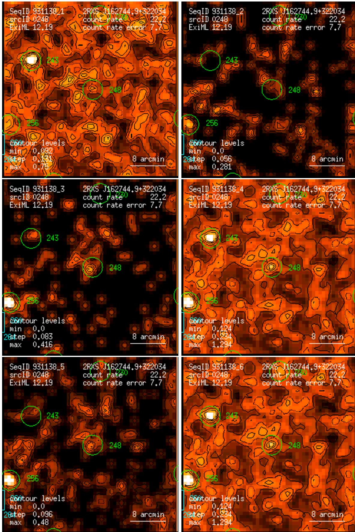
Figure 248: RASS 931138: detection 0248: band rate images, Gaussian filter: (1) PSPC channels 11 – 41, (2) 52 – 90, (3) 91 – 201, (4) 11 – 235, (5) 52 – 201, (6) 11 – 201. Broad band rates in counts/ks. Band rate contour levels in counts/ks/arcmin 2 .
